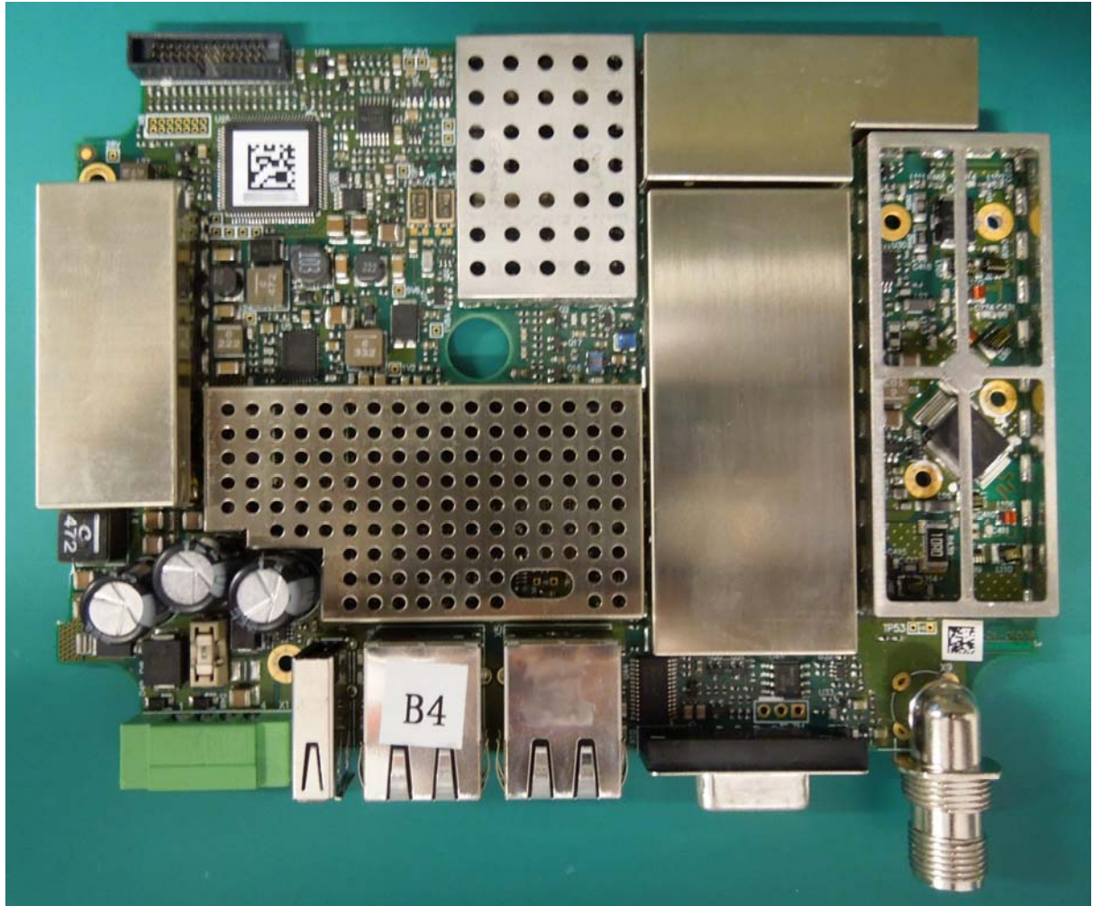
PCB top with shields
