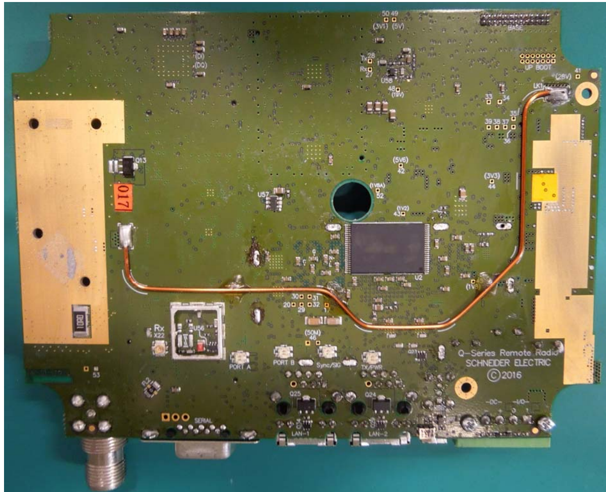
PCB bottom no shields
