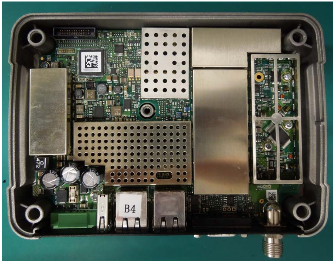
QR internal with shields
