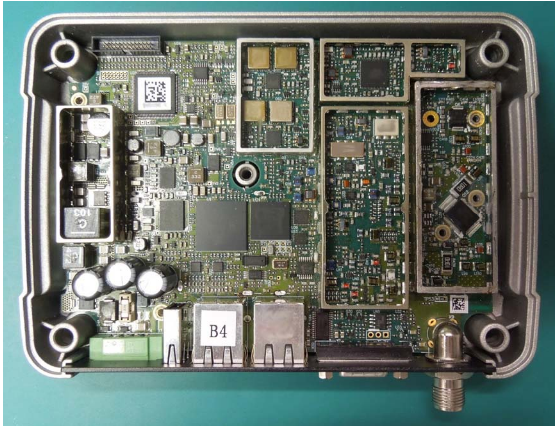
QR internal with shields
