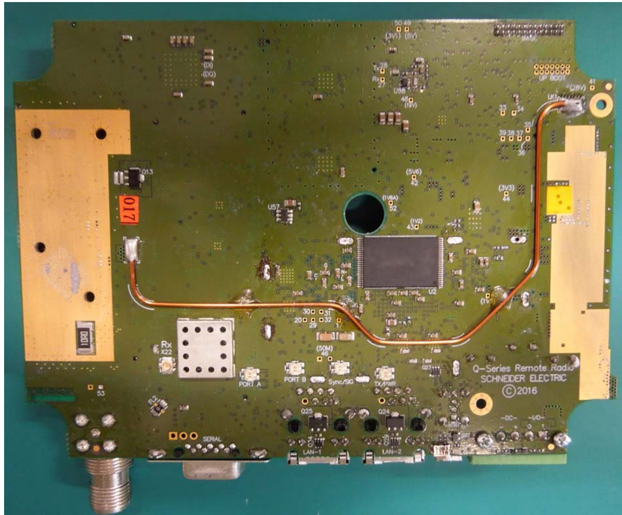
PCB bottom with shields
