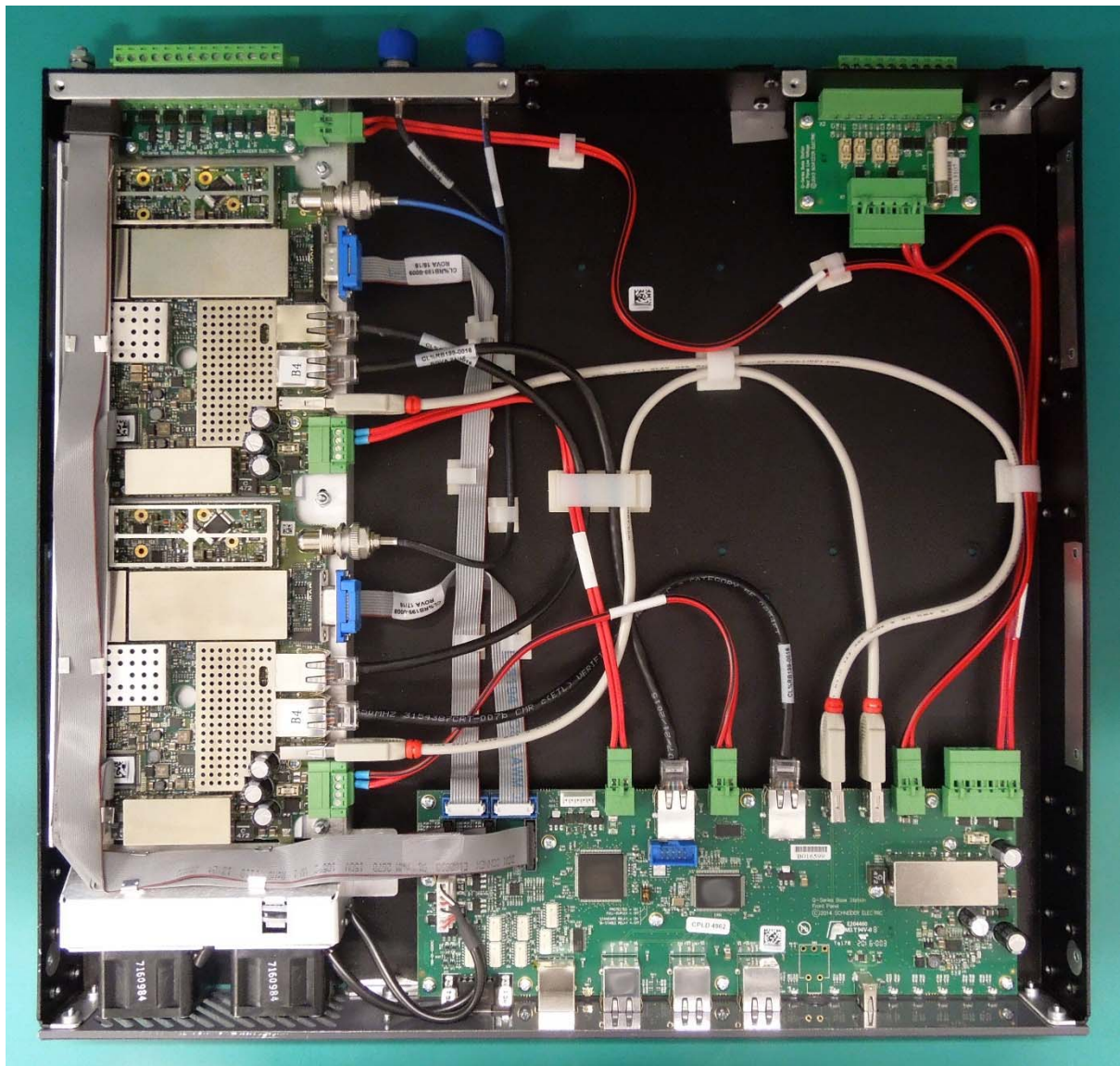
Internal view with shields
