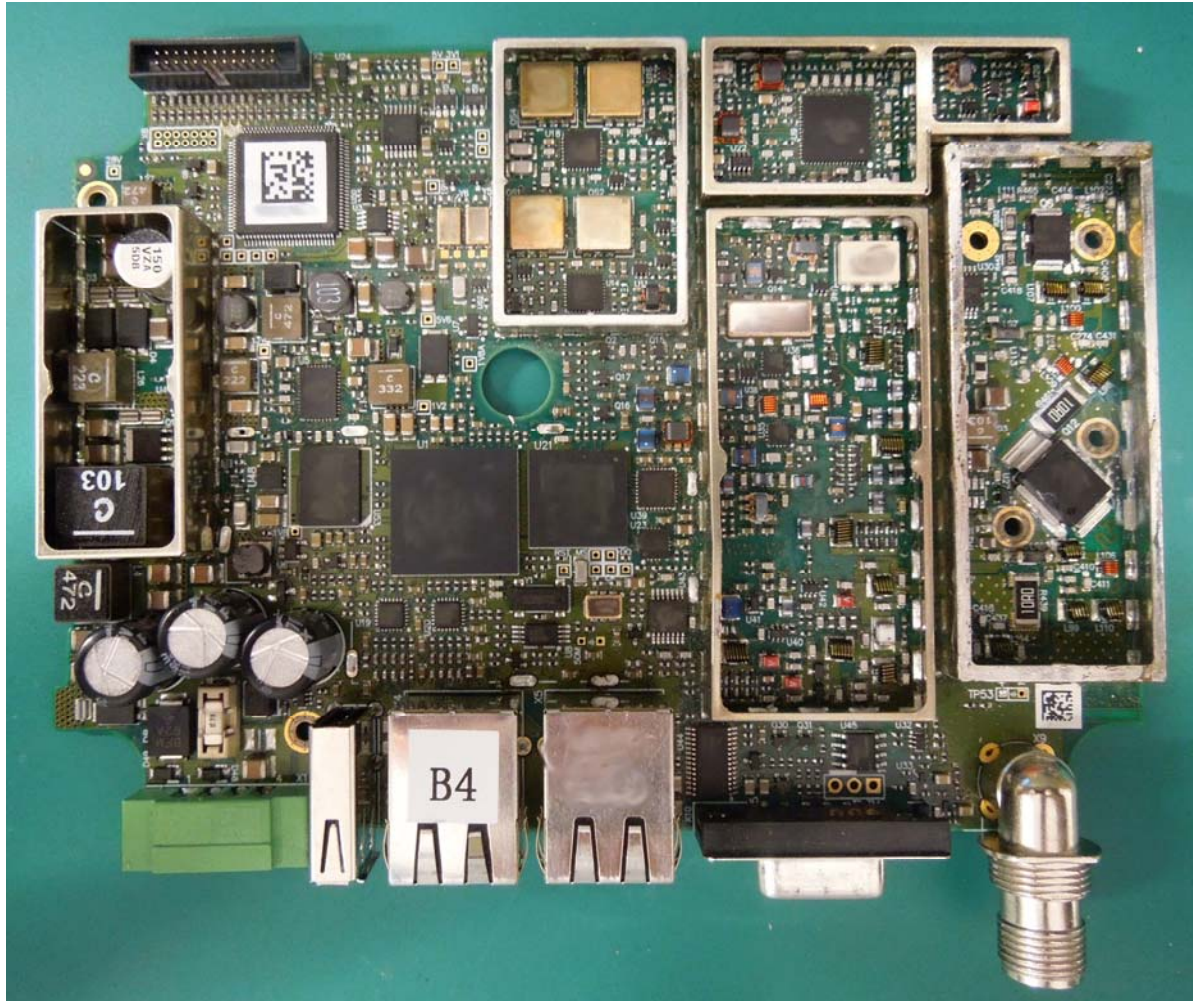
PCB top no shields
