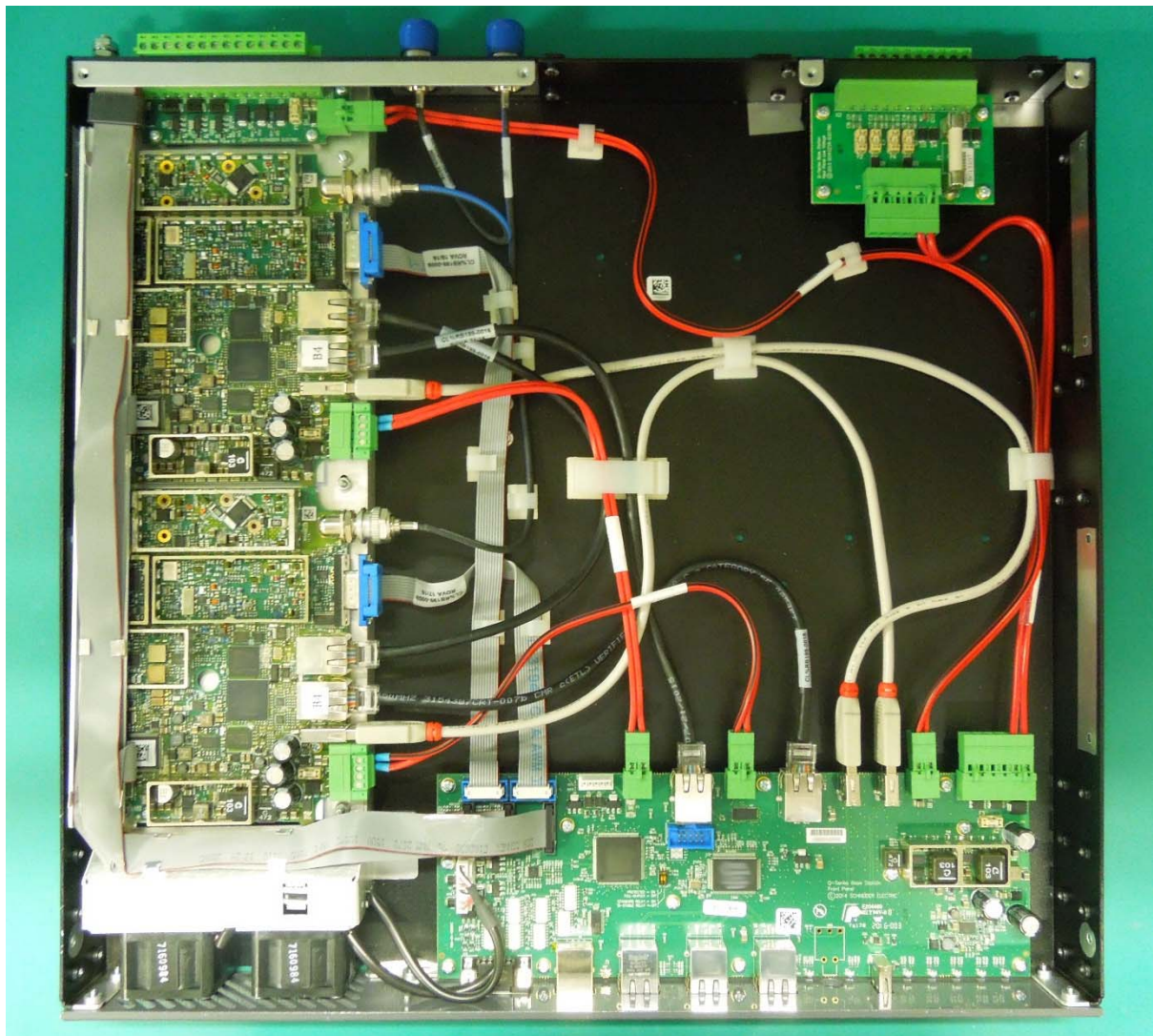
Internal view with no shields
