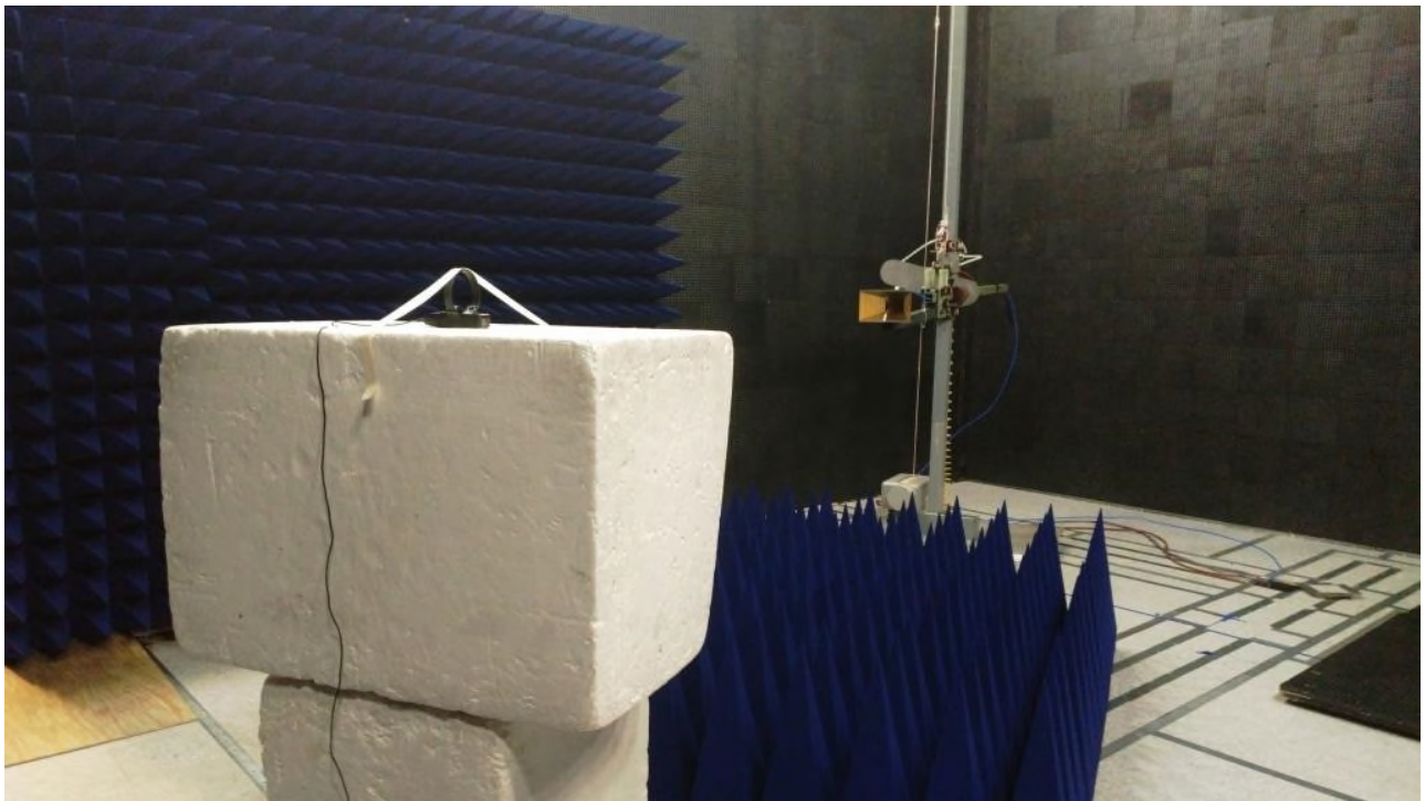
Figure 7: Equipment Under Test – Radiated Emissions >1GHz
