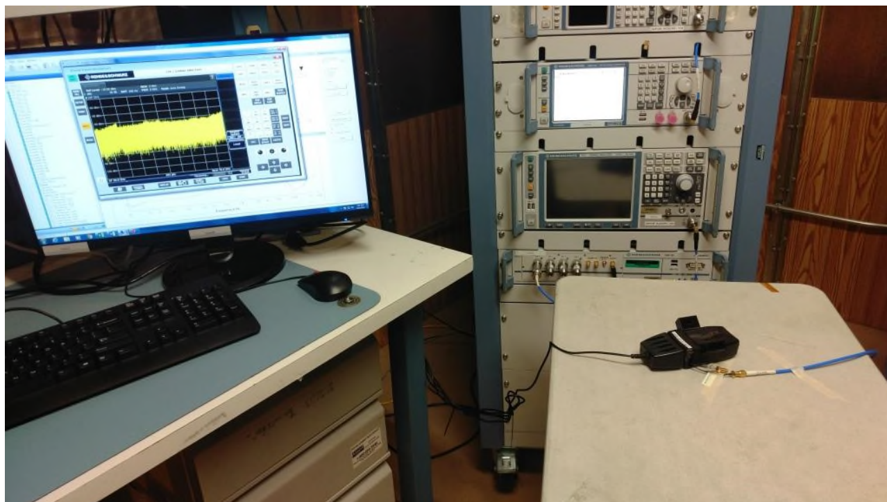
Figure 1: Equipment Under Test – Antenna Port Conducted Measurements
