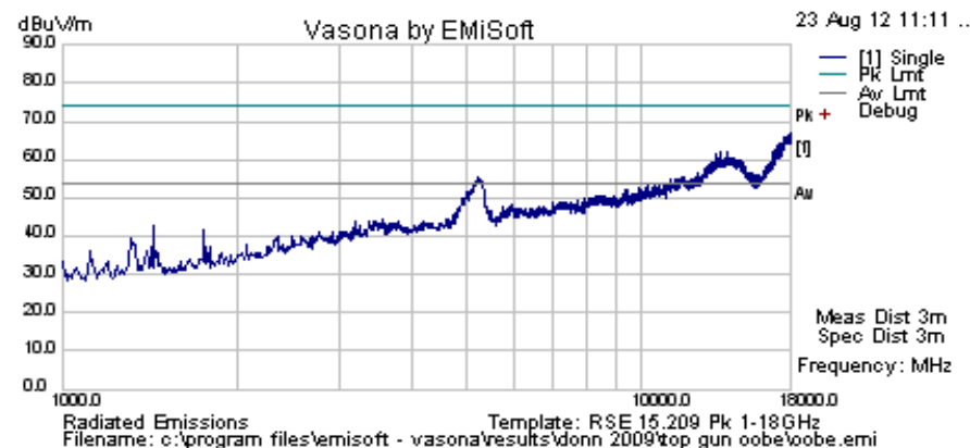
5500 HT40 PEAK
