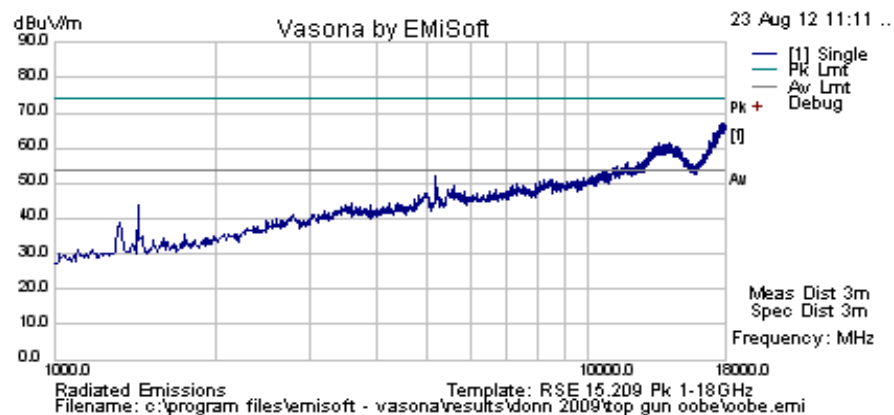
5180 OFDM PEAK
