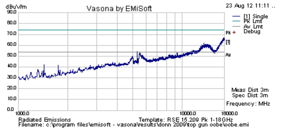
5320 HT40 PEAK
