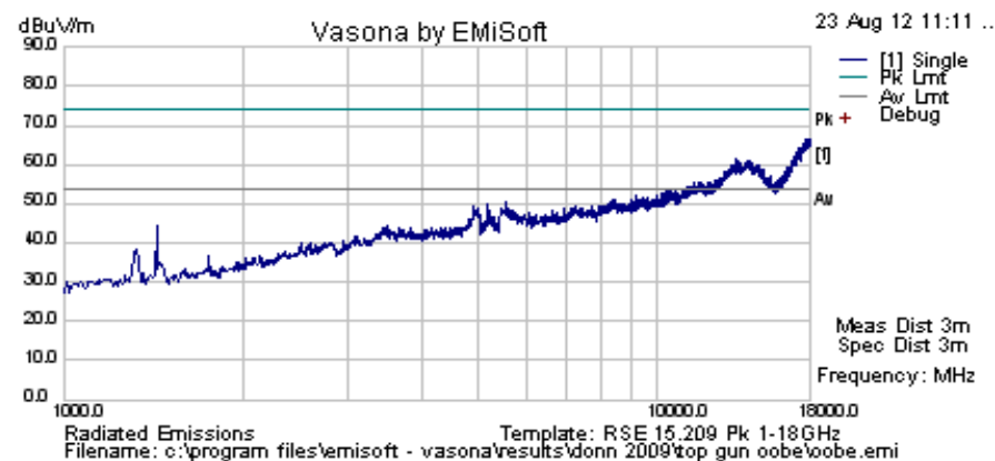
5180 HT40 PEAK
