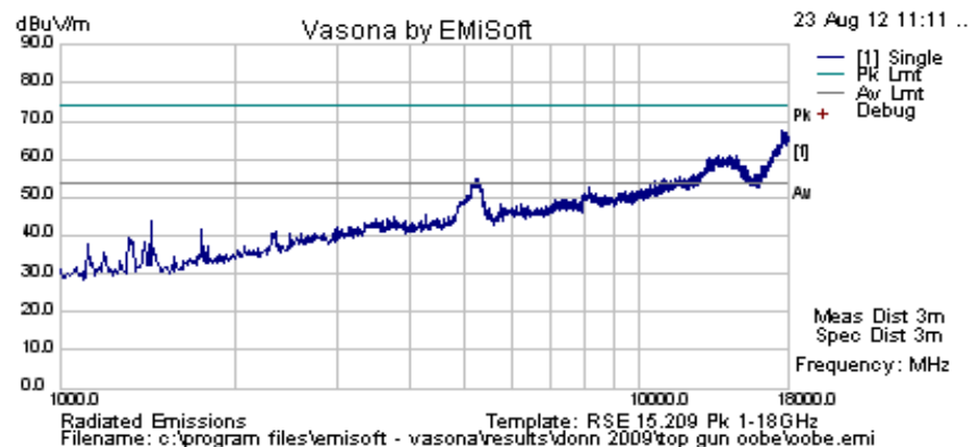
5500 OFDM PEAK
