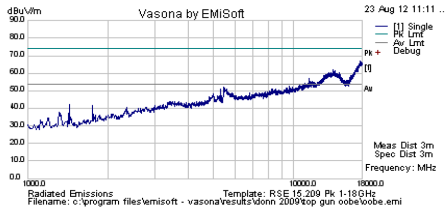
5320 OFDM PEAK
