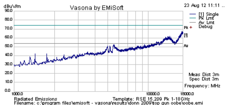
5180 HT40 PEAK
