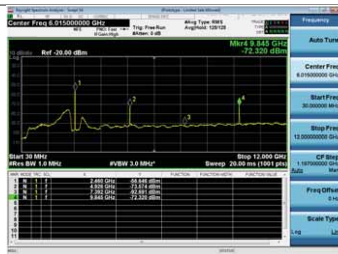
Antenna D
