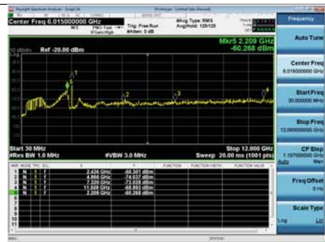
Antenna D
