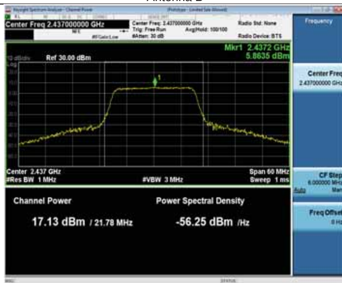
Antenna D
