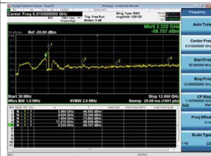
Antenna D
