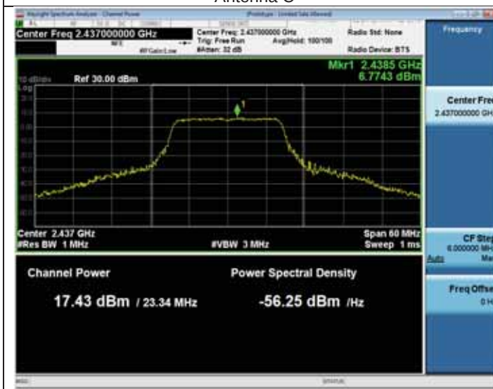
Antenna C
