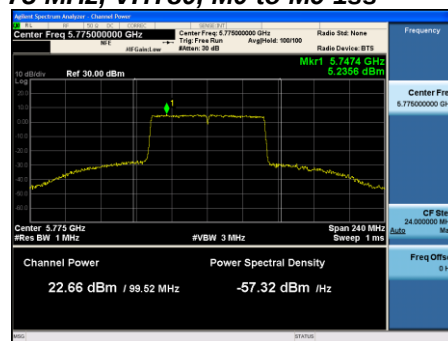
Antenna B
