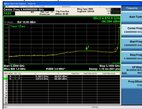
Antenna B
