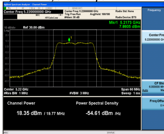
Antenna B
