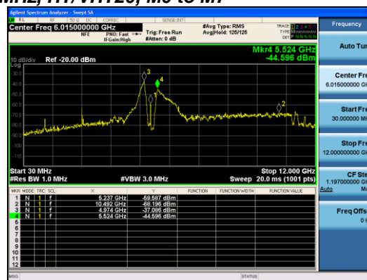
Antenna B
