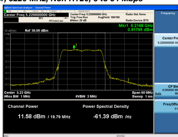
Antenna B
