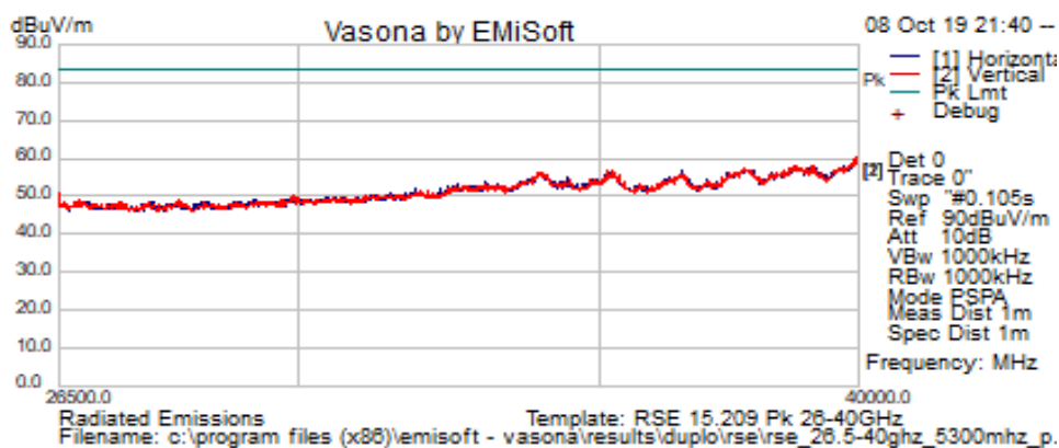
Title: TX Spurious Emissions from 26.5GHz-40GHz – Ch60 (5300 MHz)
