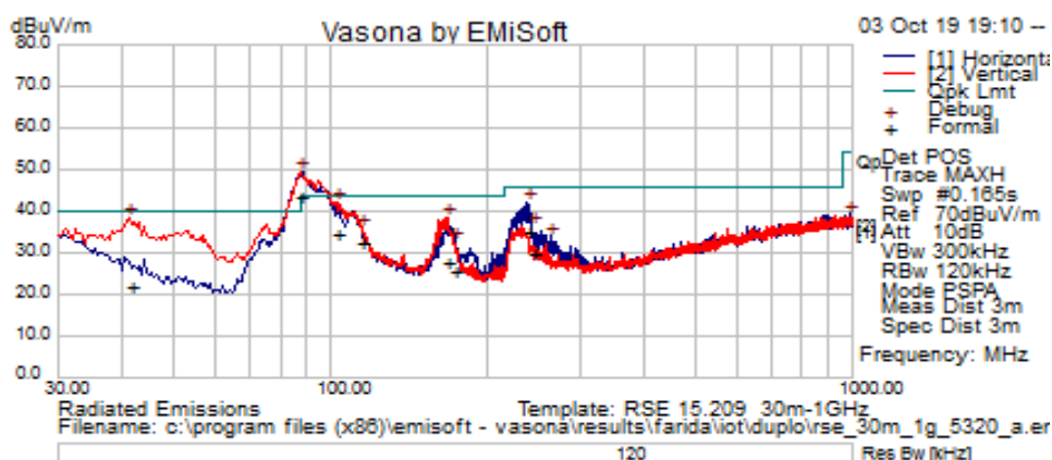
Title: TX Spurious Emissions from 30MHz-1GHz – Ch64 (5320 MHz)
