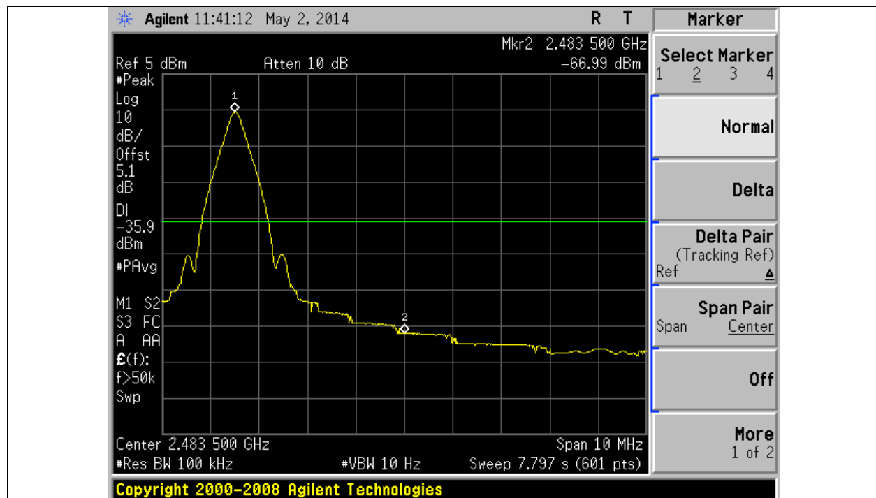
Title: Upper Band Edge Average -Hopping function off with GFSK modulation (DH5)
