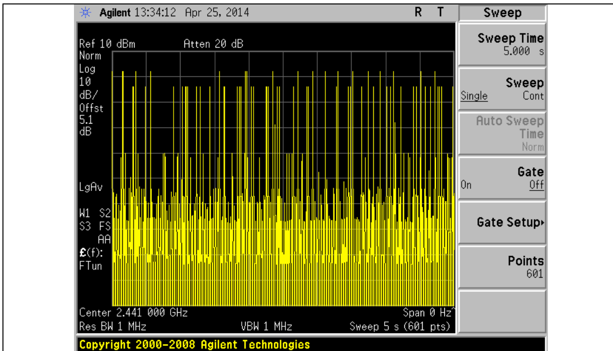
Title: Time Occupancy in 5s with 2-DH3 packet; Total bins in 5s = 19
