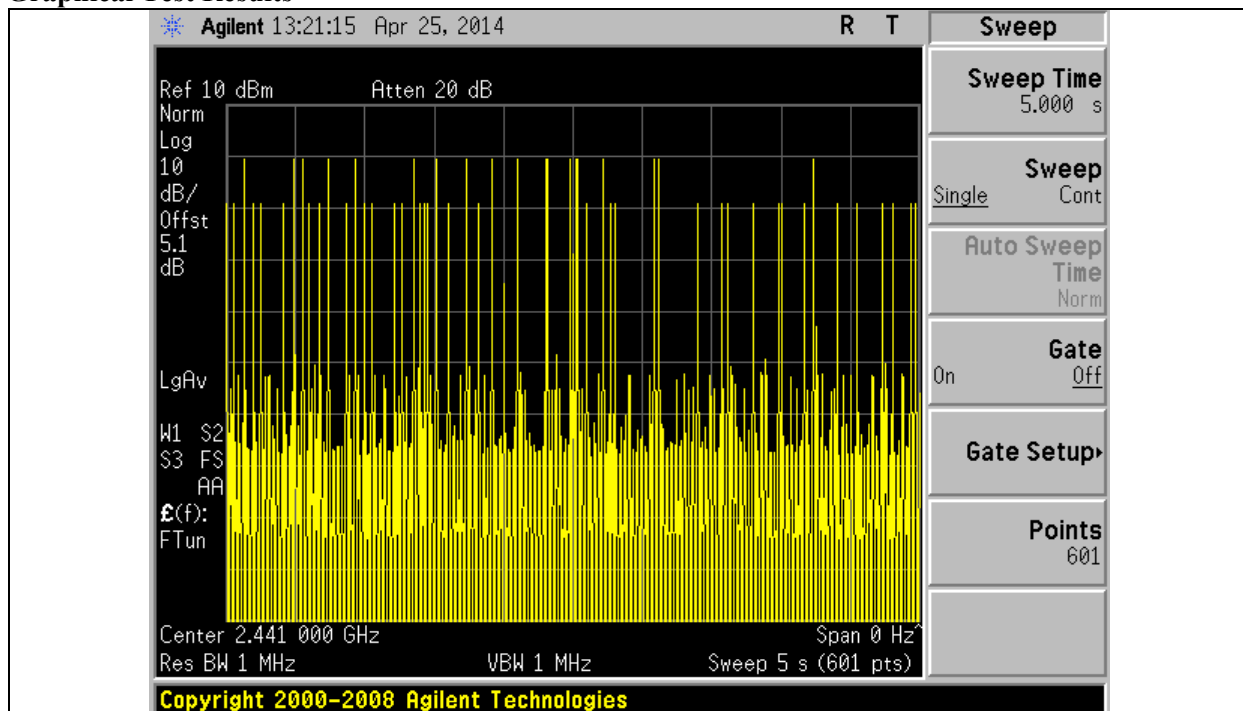
Title: Time Occupancy in 5s with DH3 packet; Total bins in 5s = 19
