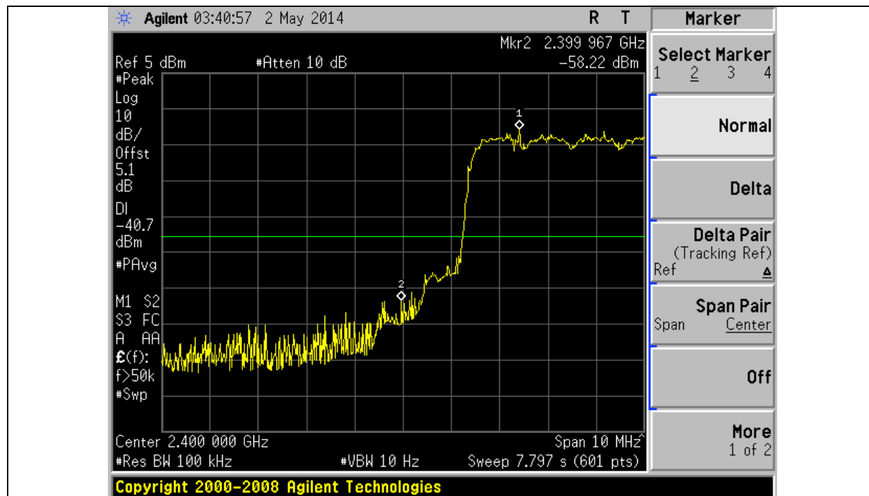
Title: Lower Band Edge Average -Hopping function on \pi/4 DQPSK modulation (2-DH5)
