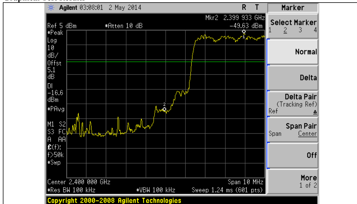
Title: Lower Band Edge Peak -Hopping function on with \pi/4 DQPSK modulation (2-DH5)
