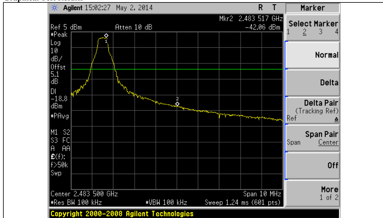
Title: Upper Band Edge Peak -Hopping function off with GFSK modulation (DH5)
