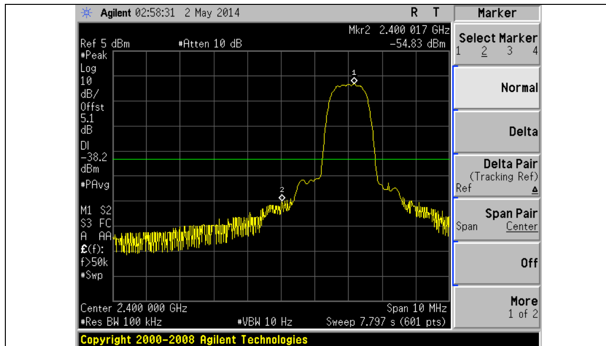
Title: Lower Band Edge Average -Hopping function off with \pi/4 DQPSK modulation (2-DH5)
