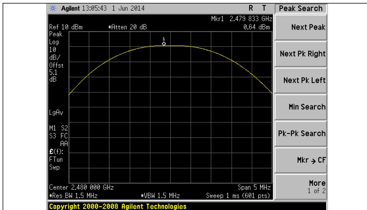
Title: Peak Output Power Ch 78: 2480MHz with GFSK modulation (DH3 packet)
