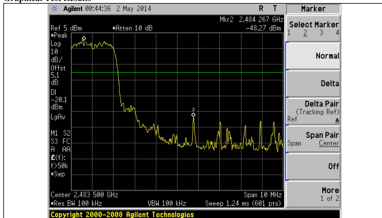
Title: Upper Band Edge Peak -Hopping function on with \pi/4 DQPSK modulation (2-DH5)
