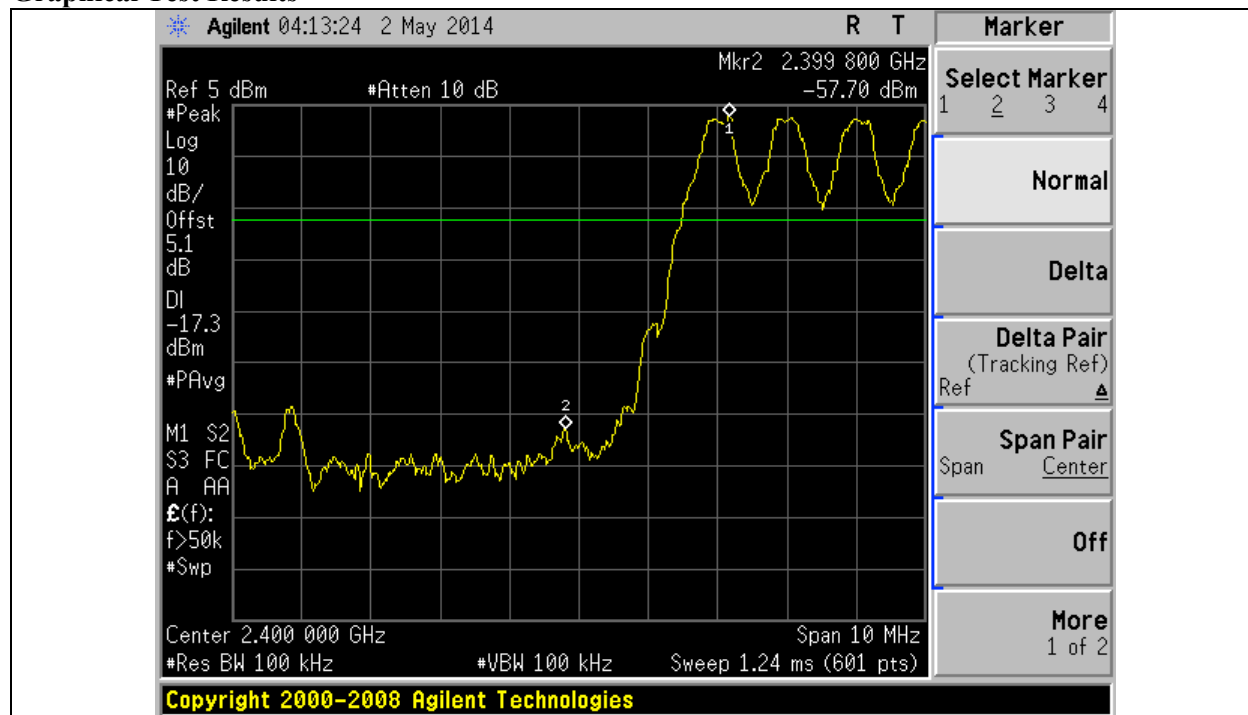
Title: Lower Band Edge Peak -Hopping function on with GFSK modulation (DH5)
