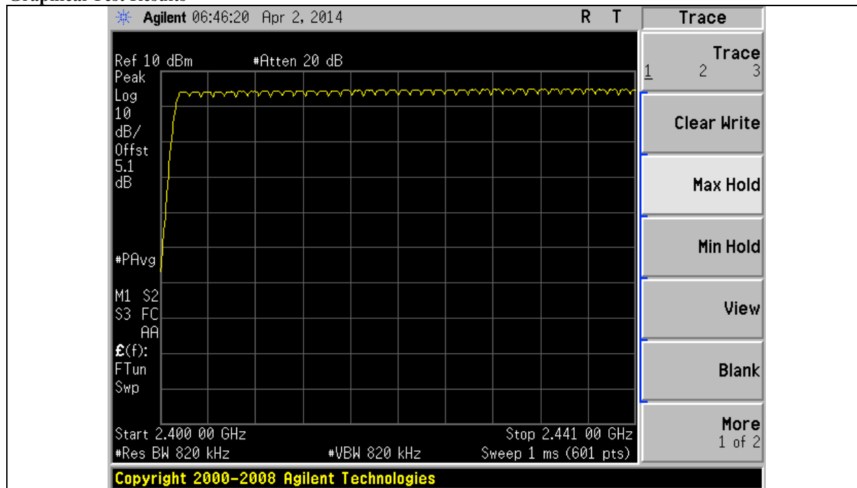
Title: Total No. of Hops Channels = 39.5 for 1 st segment in the frequency range 2400-2441MHz
