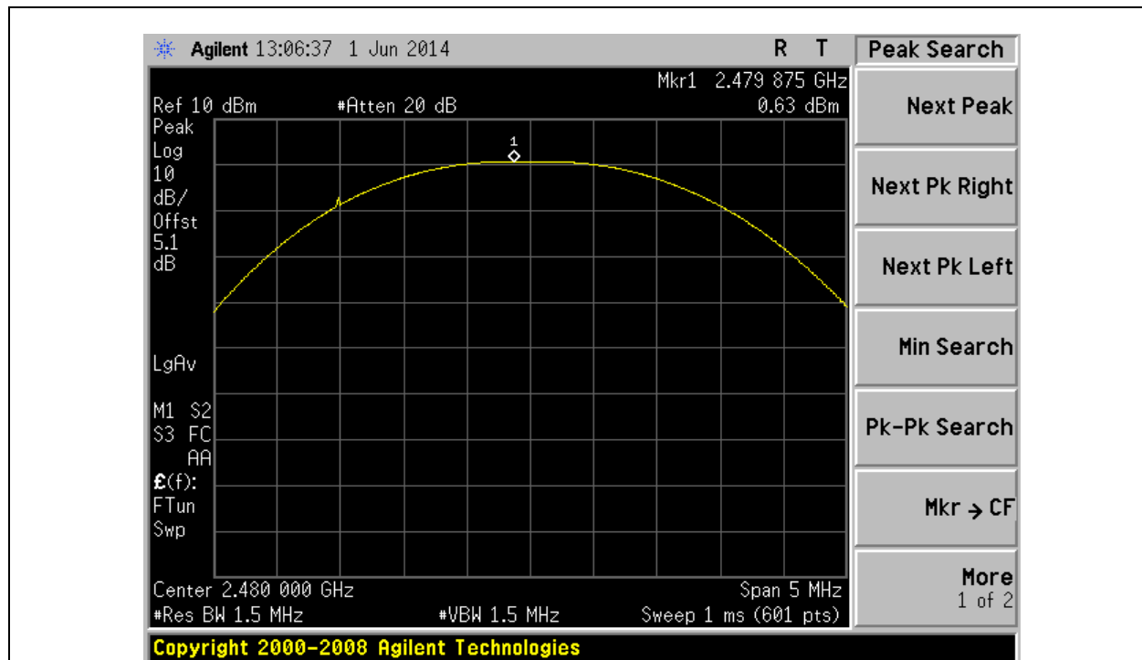
Title: Peak Output Power Ch 78: 2480MHz with GFSK modulation (DH1 packet)
