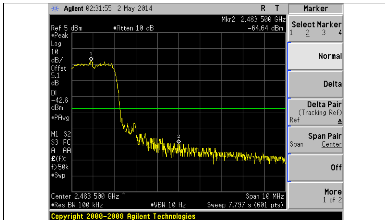
Title: Upper Band Edge Average -Hopping function on with \pi/4 DQPSK modulation (2-DH5)
