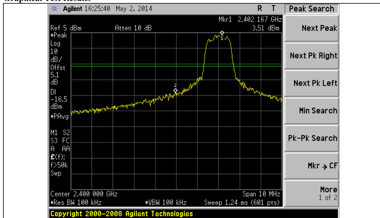
Title: Lower Band Edge Peak -Hopping function off with \pi/4 DQPSK modulation (2-DH5)
