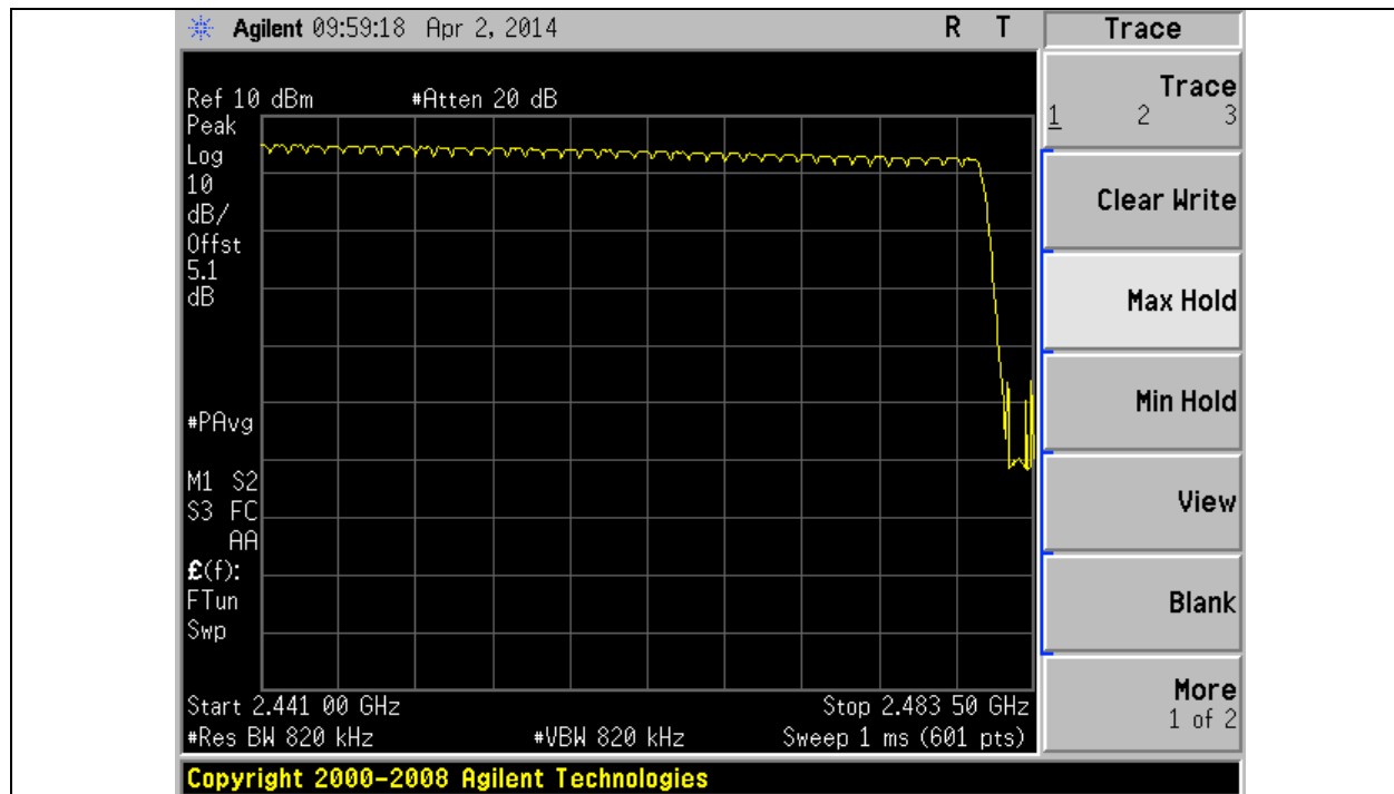
Title: Total No. of Hops Channels = 39.5 for 2 nd segment in the frequency range 2441-2483.5MHz
