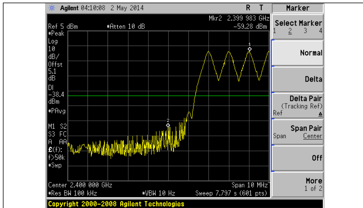
Title: Lower Band Edge Average -Hopping function on with GFSK modulation (DH5)
