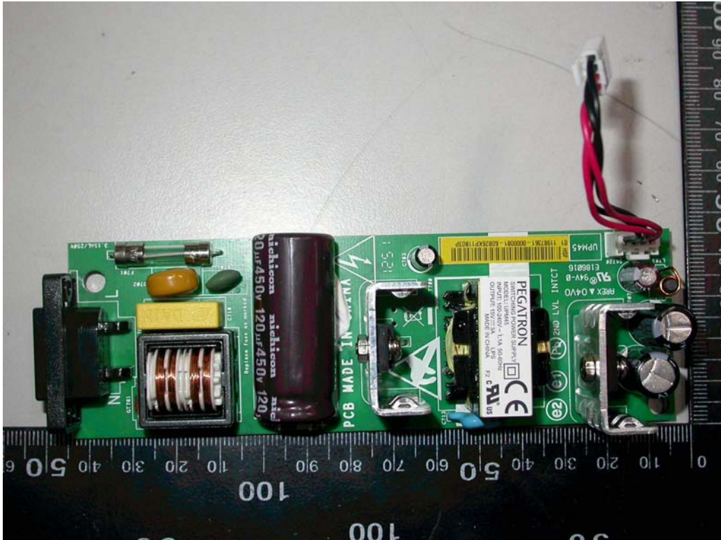
20. Front view of PCB2
