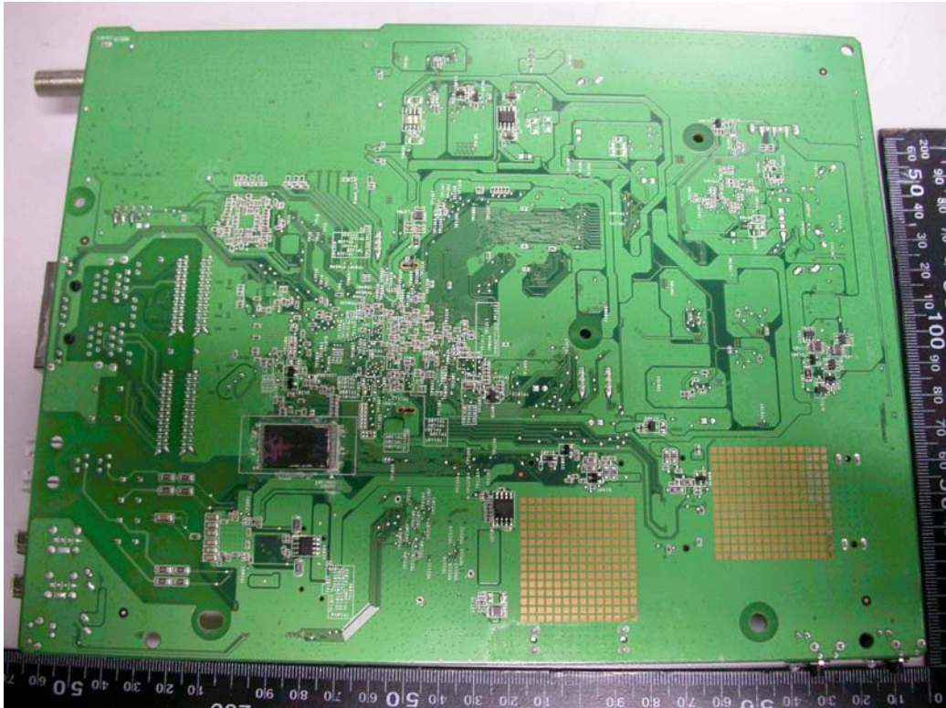
19. Rear view of PCB1
