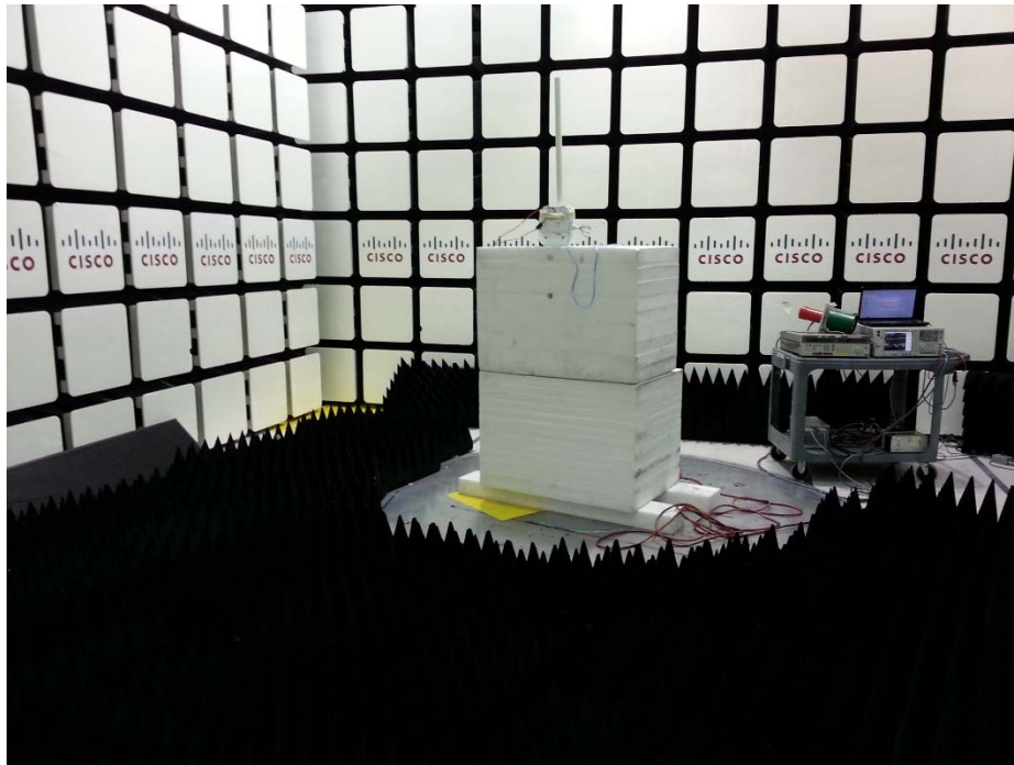
18 – 40GHz Setup
