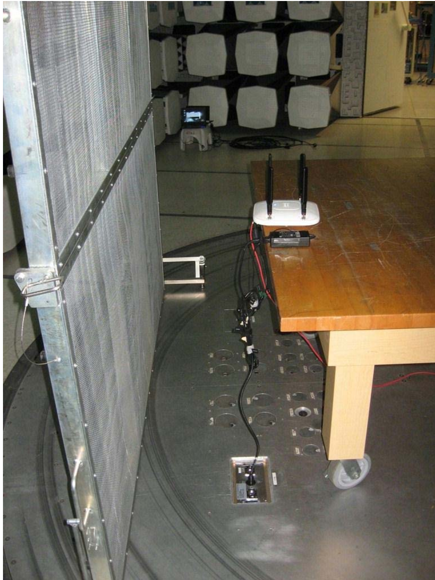
AC Conducted Emissions Setup
