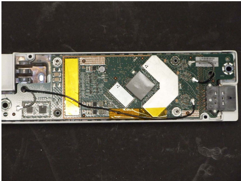
Antenna Feed Line Connections to PCB
