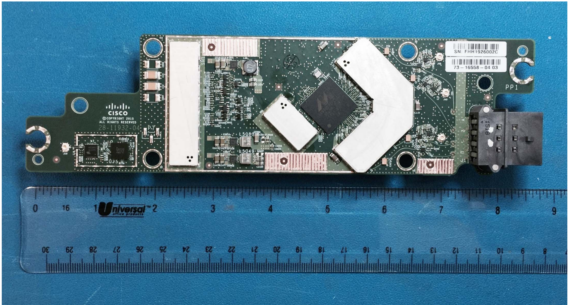
Top of board with shields
