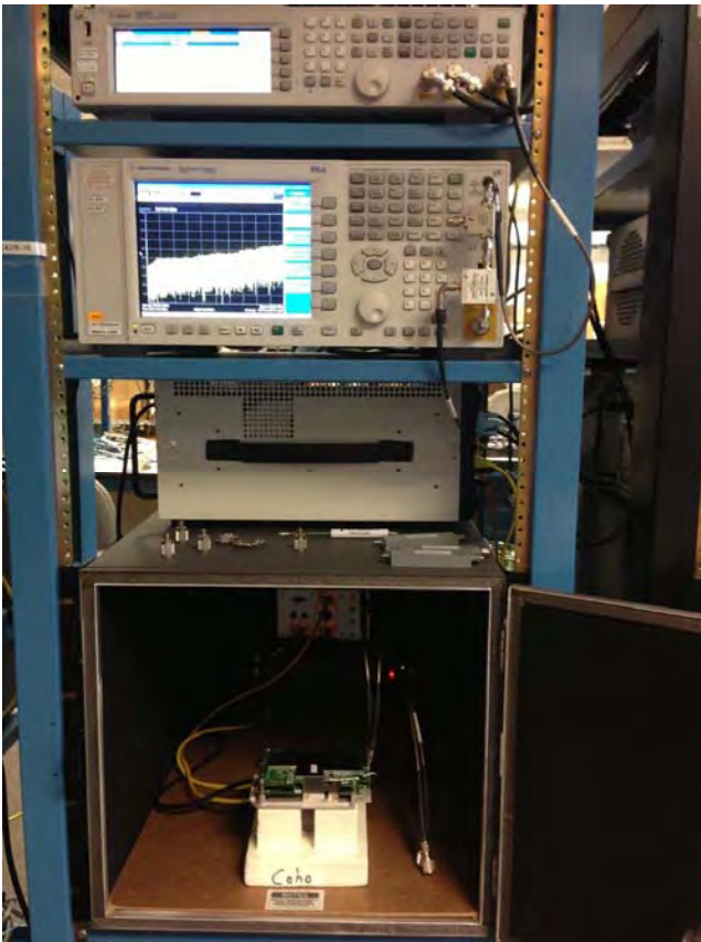
Conducted Test Setup
