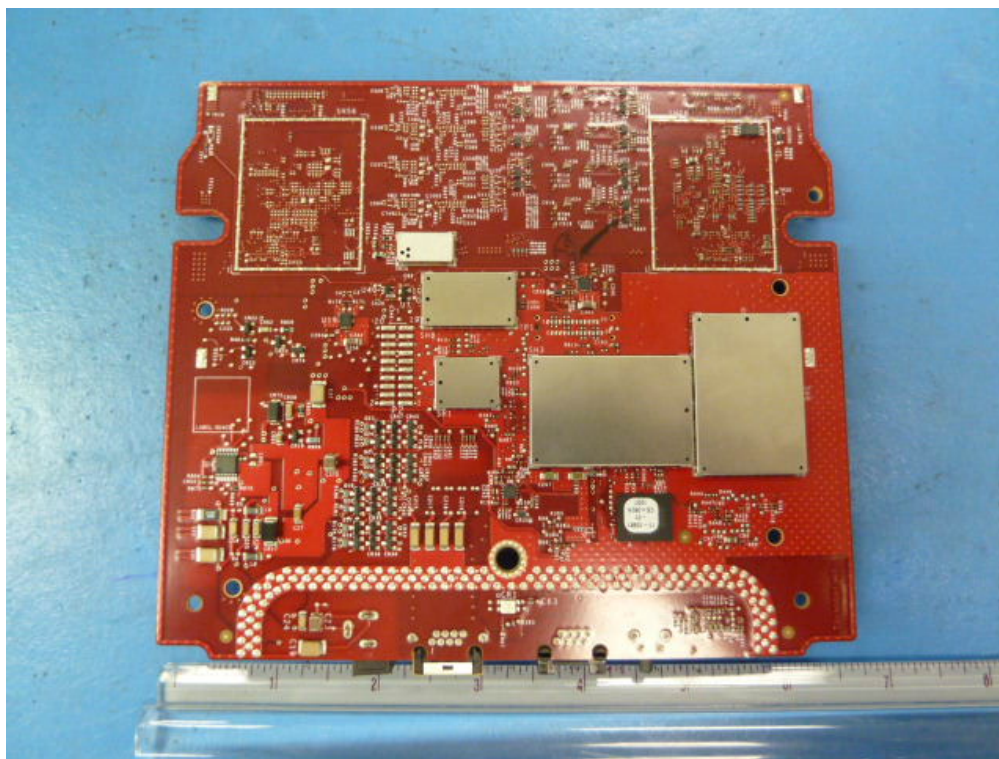
2601 Series Shielded Board Bottom
