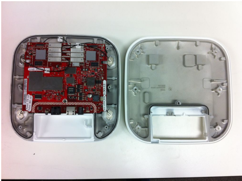
2600E Series Internal Assembly
