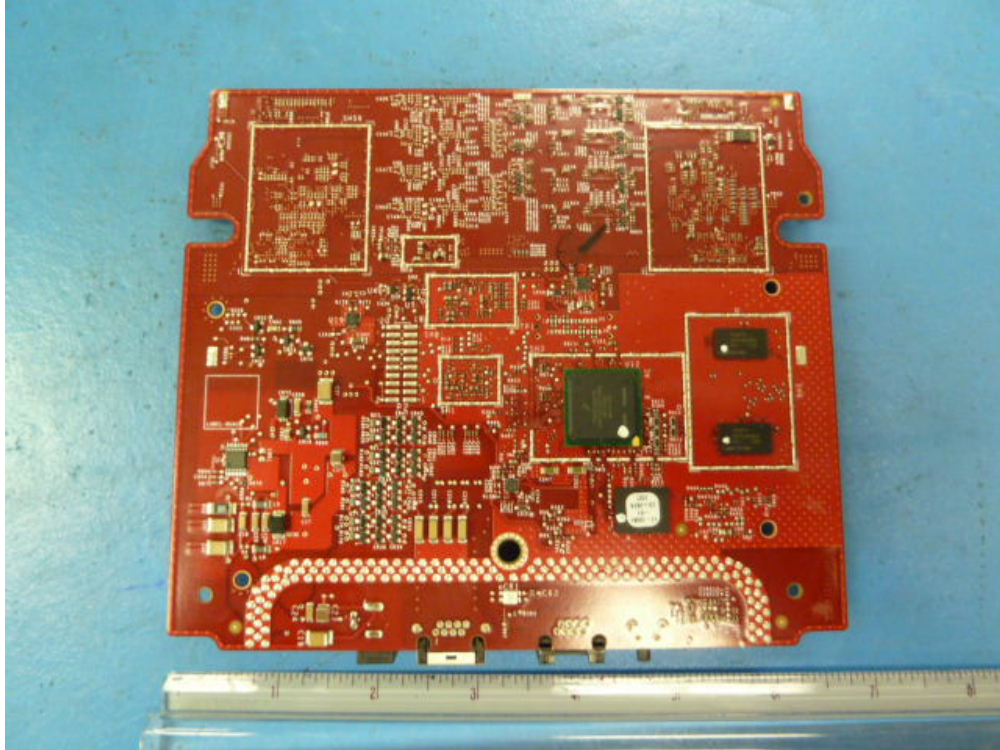
2601 Series Unshielded Board Bottom
