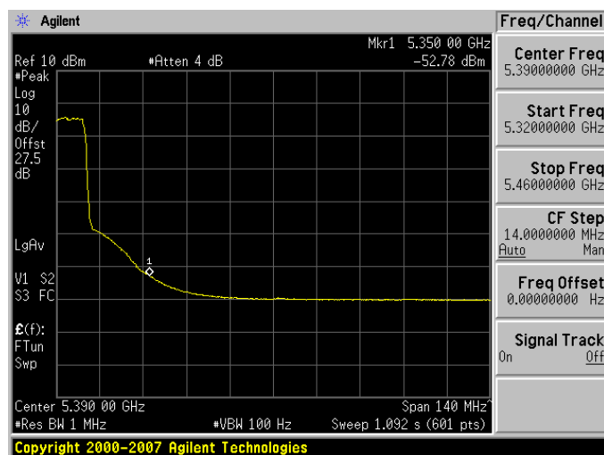
Antenna D
