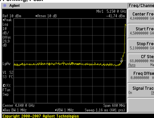
Antenna B
