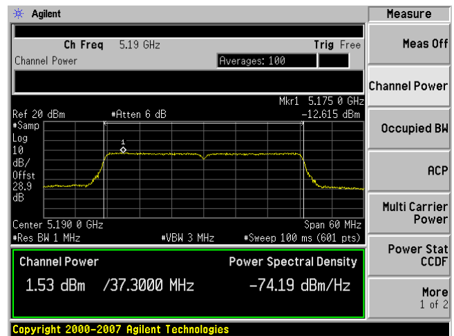
Antenna D
