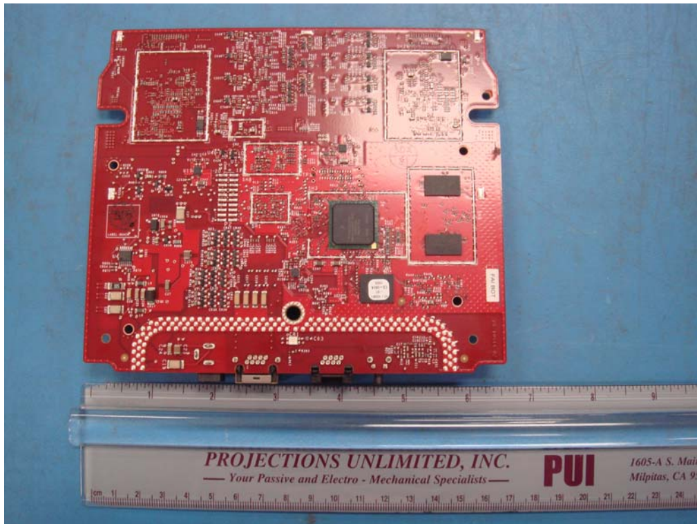
2602 Series Unshielded Board Bottom
