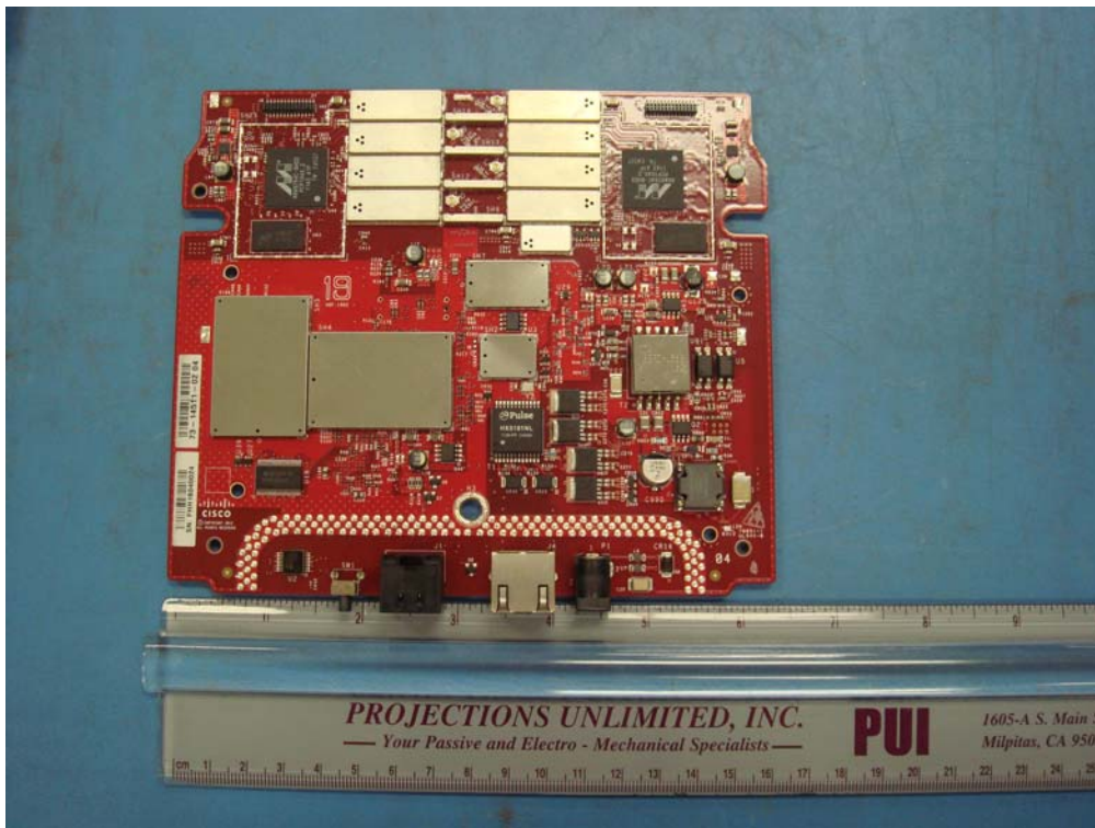
2602 Series Shielded Board Top
