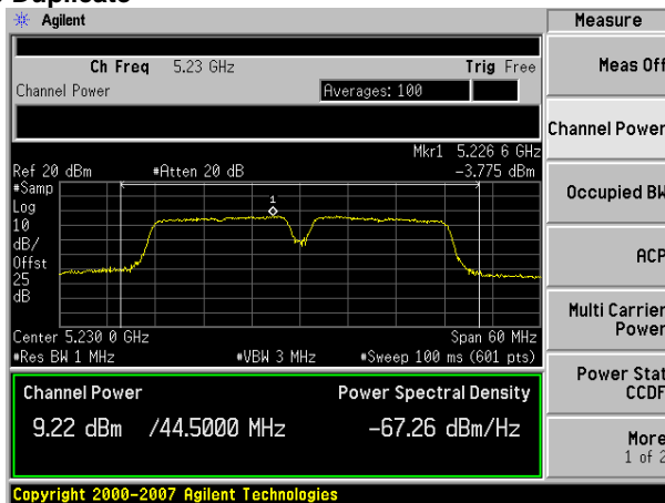
Antenna B
