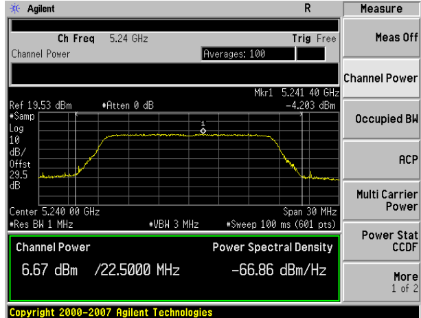
Antenna B
