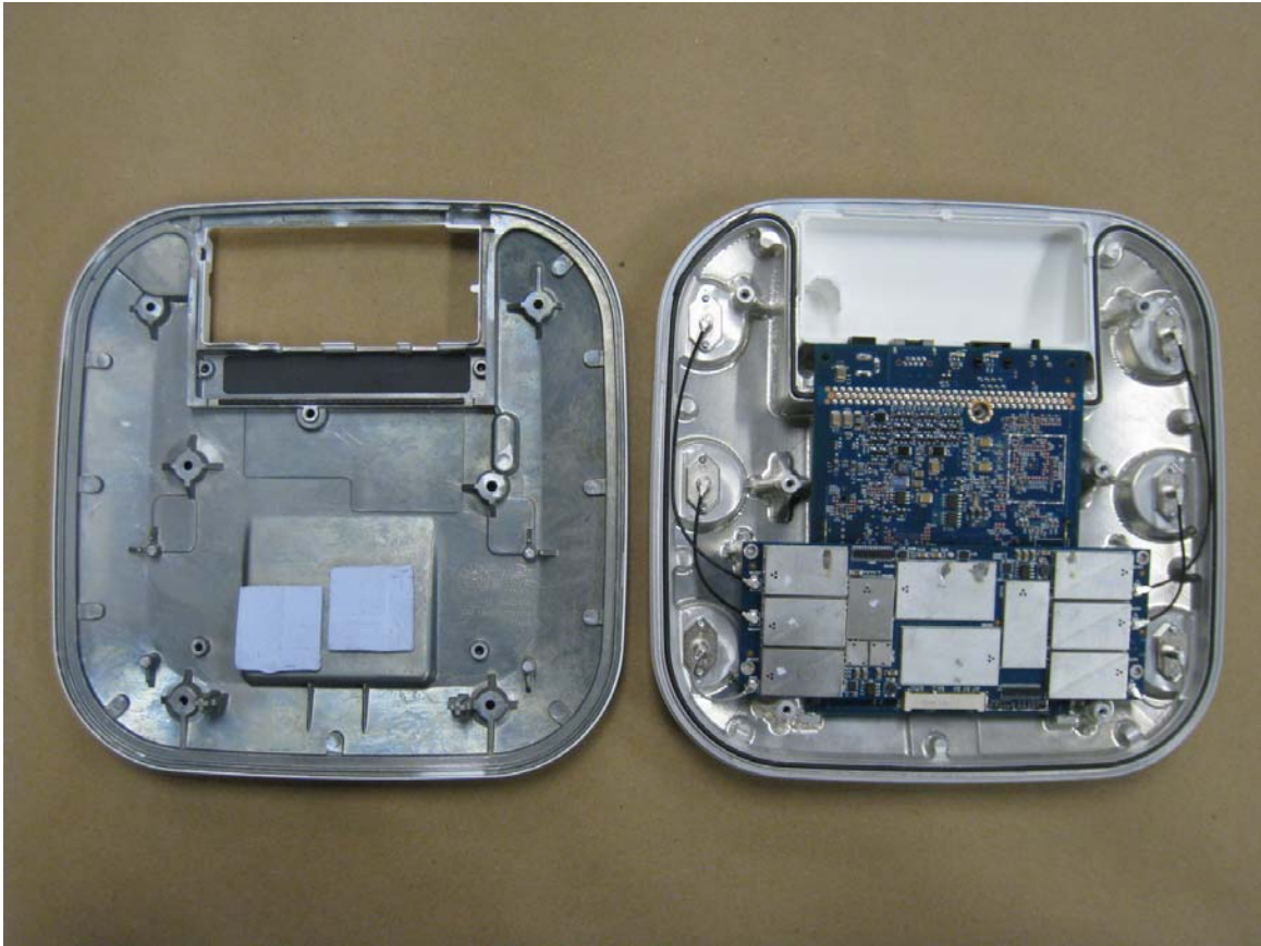
AP3502 Series Internal Photos
