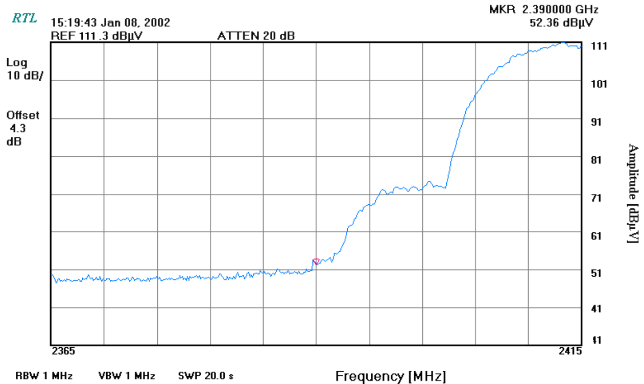
PLOT 3-6: BAND EDGE: PEAK MEASUREMENT FOR CHANNEL 1
