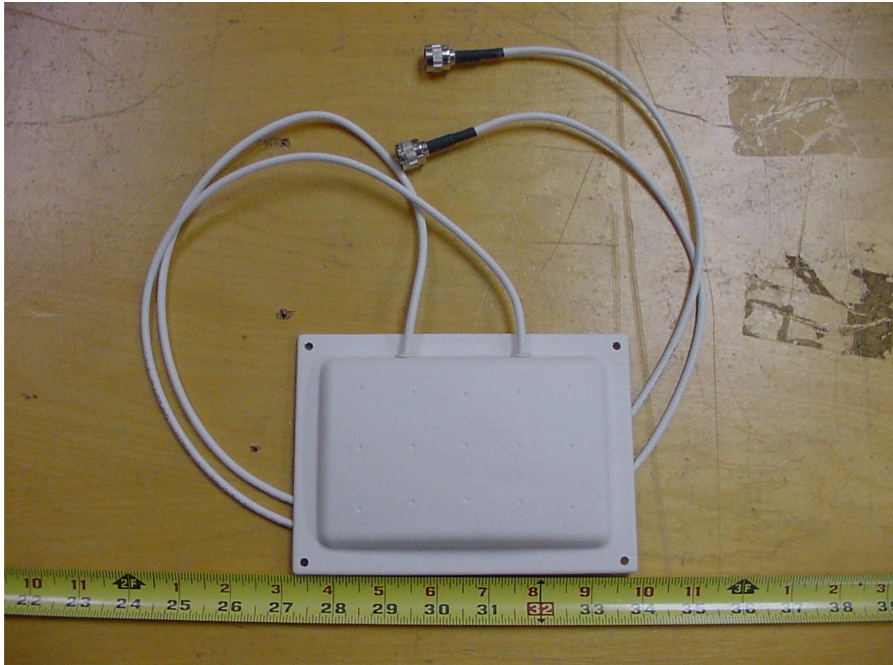
PHOTOGRAPH 6: ANTENNA AIR-ANT2012
