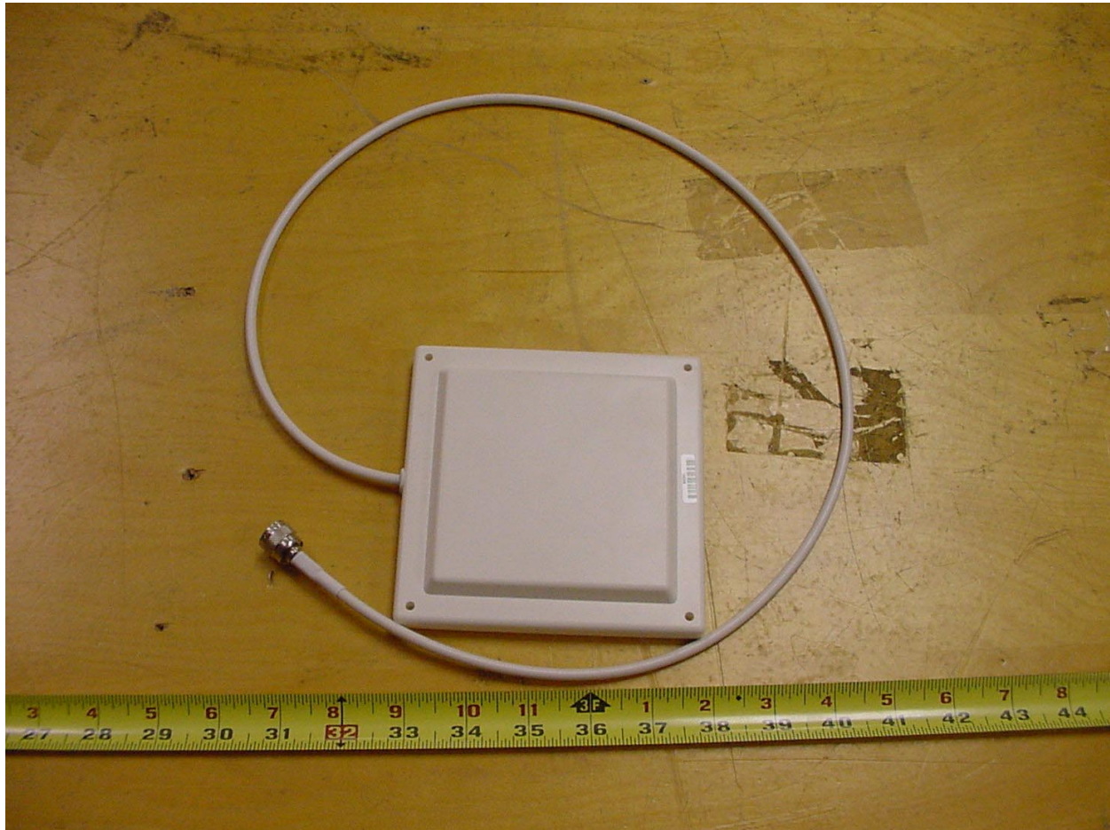
PHOTOGRAPH 5: ANTENNA AIR-ANT3549
