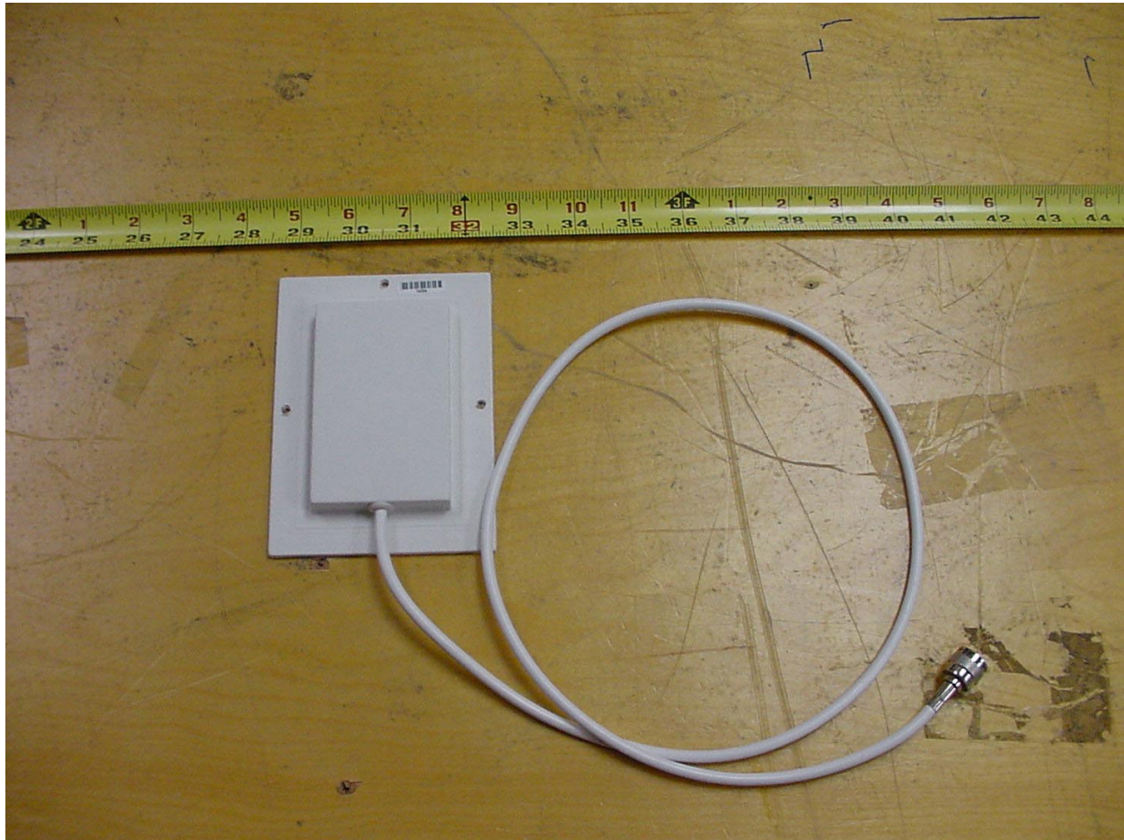
PHOTOGRAPH 7: ANTENNA AIR-ANT1729
