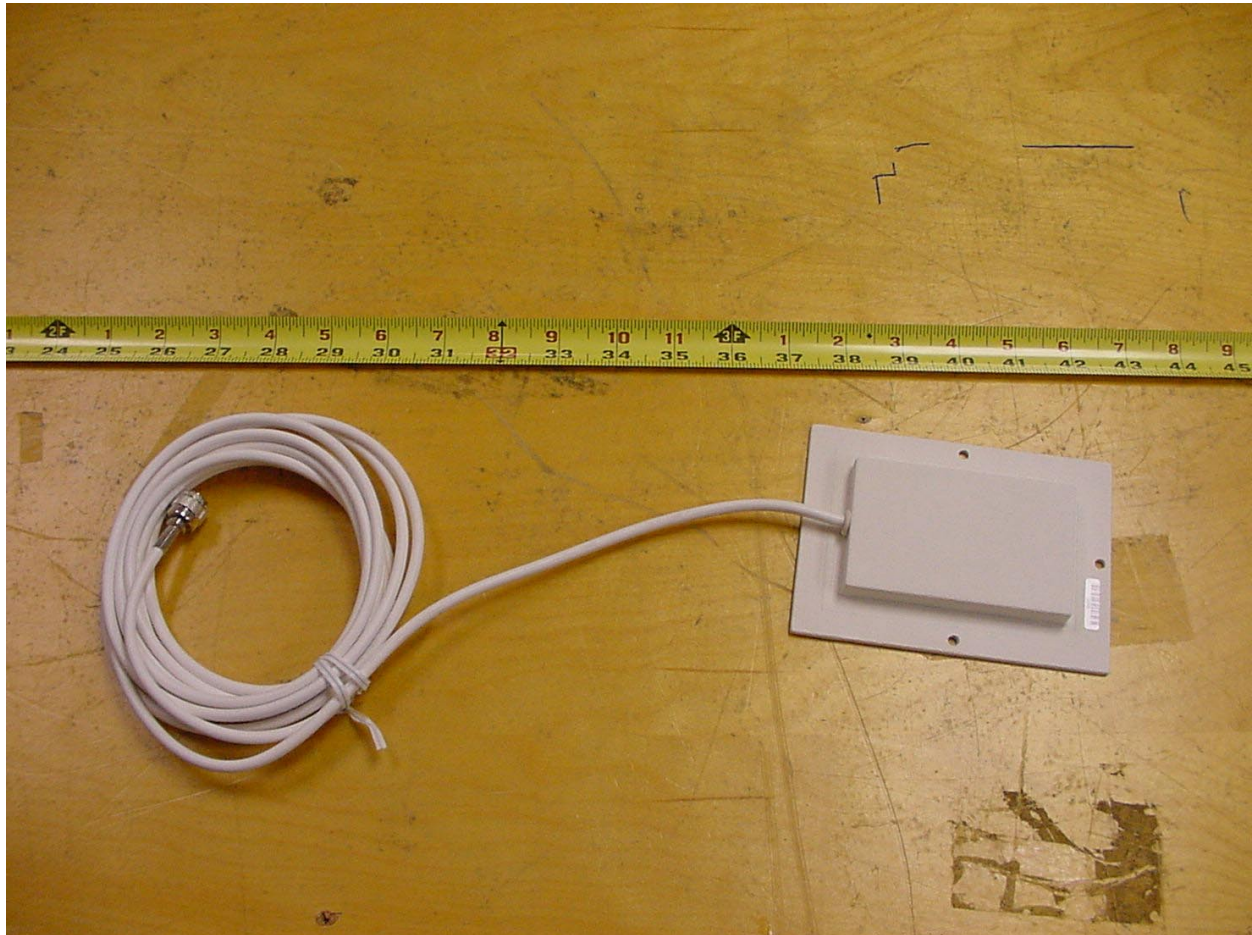
PHOTOGRAPH 10: ANTENNA AIR-ANT3195
