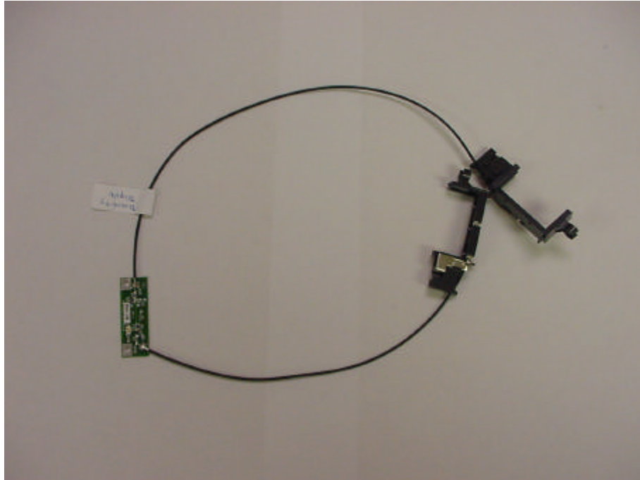
Dipole Diversity antenna
