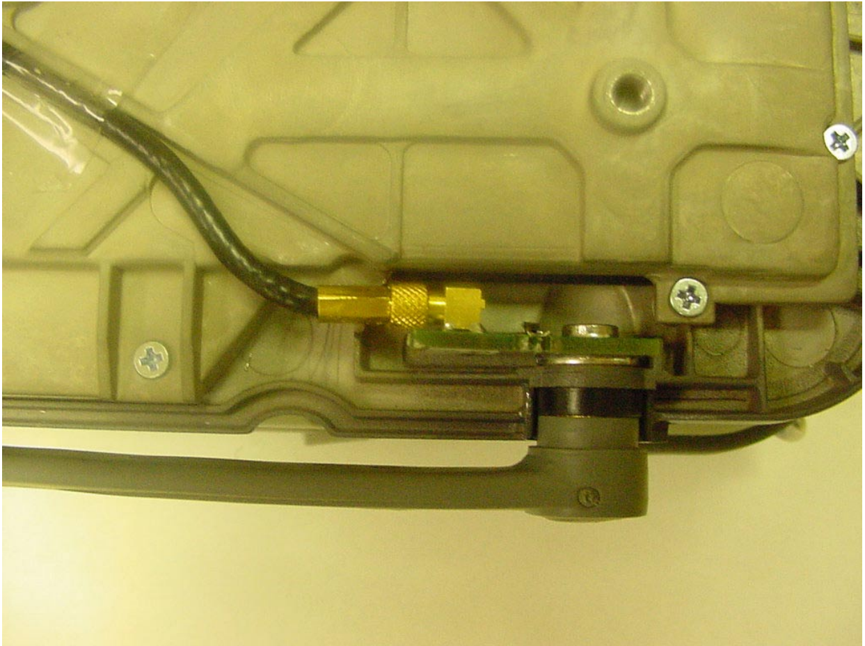
PHOTOGRAPH 16: ANTENNA CONNECTION (ITRONIX IX550)
