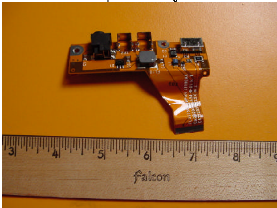
Top View of of Charger
