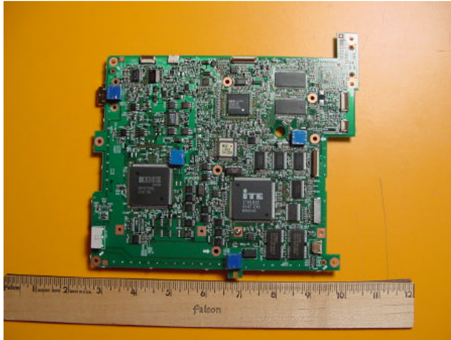
Top View of Board
