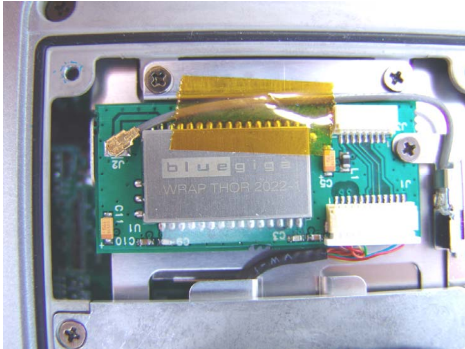
BT2022 removed to show PIFA antenna
