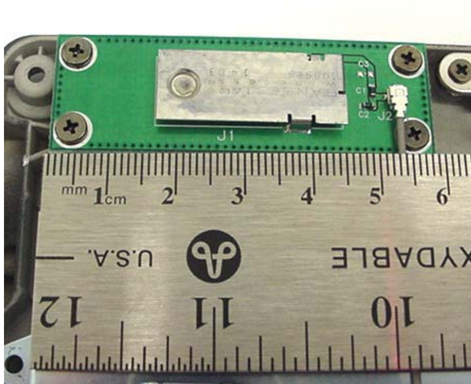
RangeStar Surface-Mount Antenna P/N: 100929 (WLAN)
