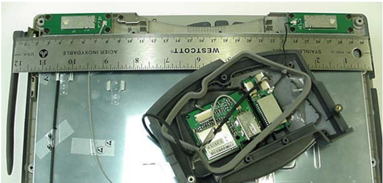
WLAN Surface-Mount Antenna (Upper Right Side Rear Edge of LCD Display)
