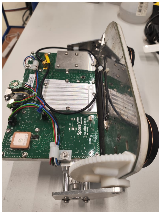
Photo 18: SpaceCom Class 7 Antenna
