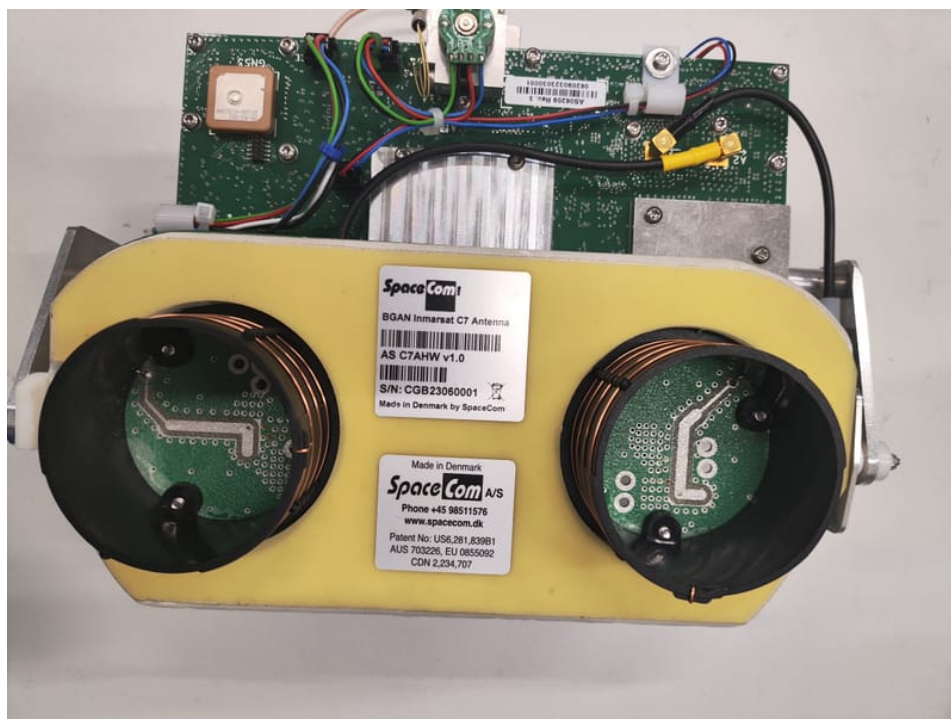
Photo 15: SpaceCom Class 7 Antenna
