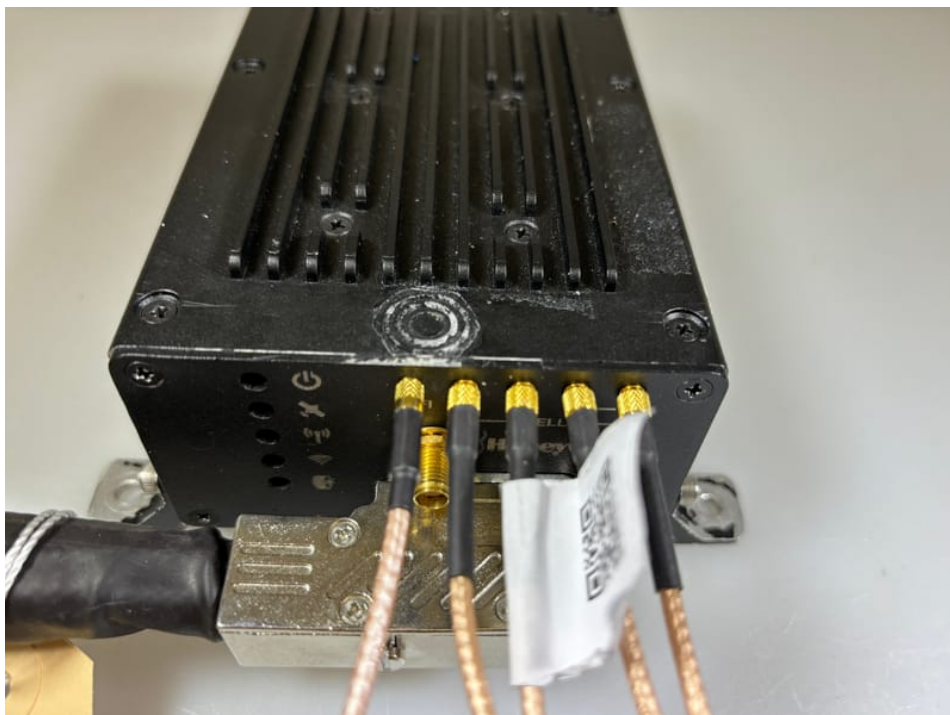
Photo 8: EUT with cellular and WLAN antennas
