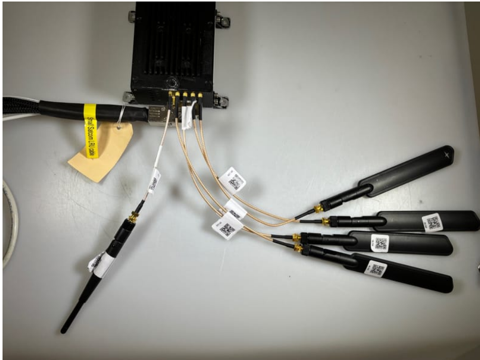
Photo 7: EUT with cellular and WLAN antennas
