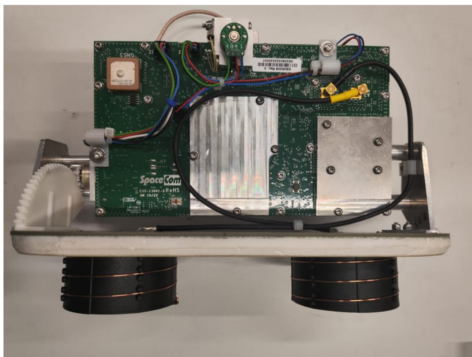
Photo 16: SpaceCom Class 7 Antenna
