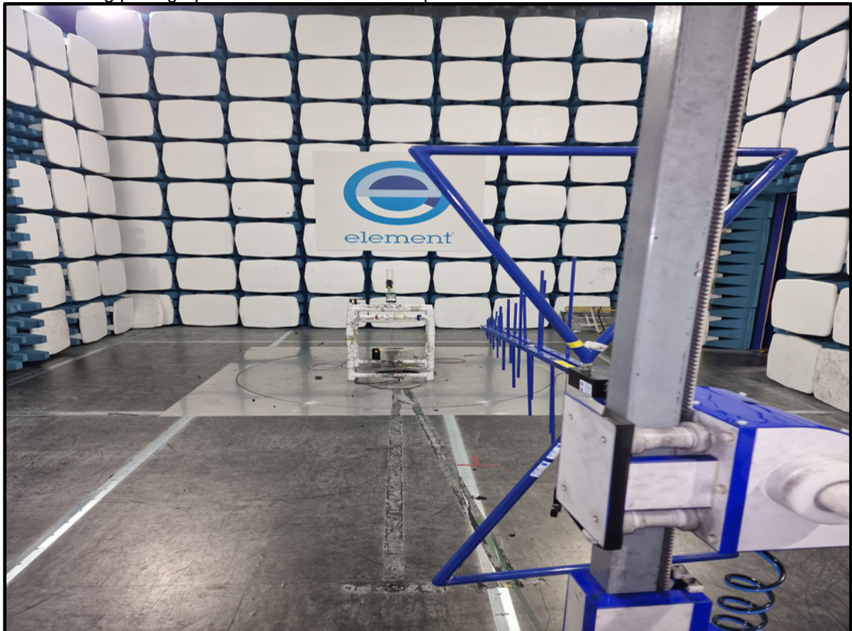
Radiated Test Setup < 1 GHz
