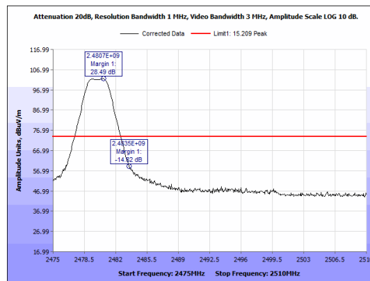
Figure 32: Radiated Restricted Band Edge Peak. IEEE 15.4 High Channel
