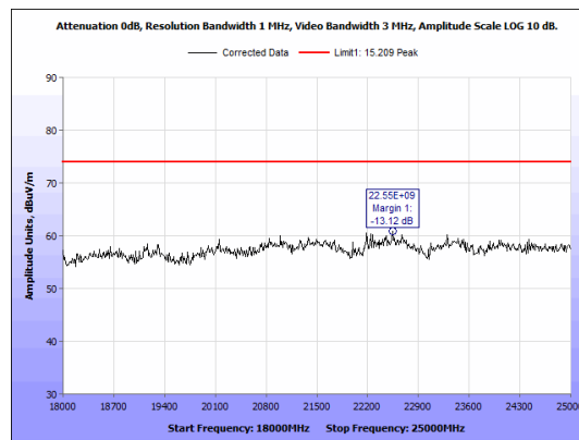
Figure 29: Radiated Emission Peak. BLE 1 Mbps Low Channel 18GHz-25GHz
