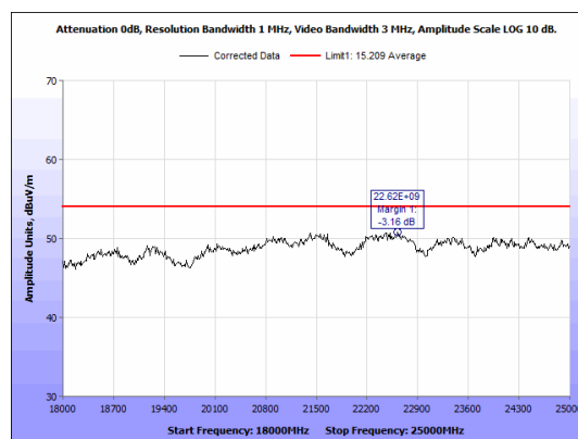
Figure 33: Radiated Emission Average. BLE 1 Mbps Mid Channel 18GHz-25GHz
