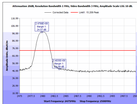
Figure 58: Restricted Band Edge Peak. BLE 1 Mbps High Channel
