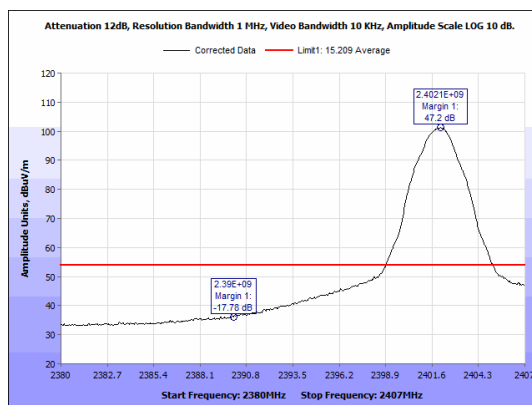
Figure 59: Restricted Band Edge Average. BLE 2 Mbps Low Channel
