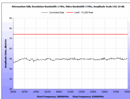
Figure 54: Radiated Emission Peak. BLE 2 Mbps High Channel 18GHz-25GHz
