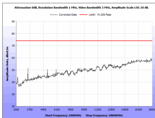
Figure 47: Radiated Emission Peak. BLE 2 Mbps Mid Channel 1GHz-18GHz
