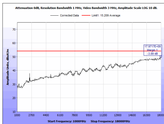
Figure 36: Radiated Emission Average. BLE 1 Mbps High Channel 1GHz-18GHz
