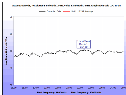
Figure 38: Radiated Emission Average. BLE 1 Mbps High Channel 18GHz-25GHz
