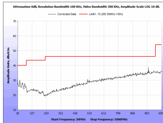
Figure 40: Radiated Spurious Emission. BLE 2 Mbps Low Channel 30MHz-1GHz
