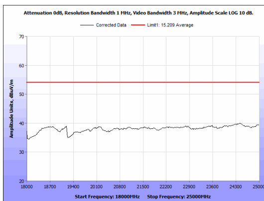
Figure 53: Radiated Emission Average. BLE 2 Mbps High Channel 18GHz-25GHz
