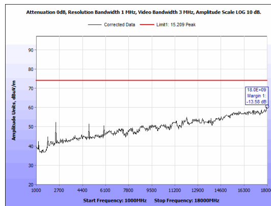
Figure 32: Radiated Emission Peak. BLE 1 Mbps Mid Channel 1GHz-18GHz
