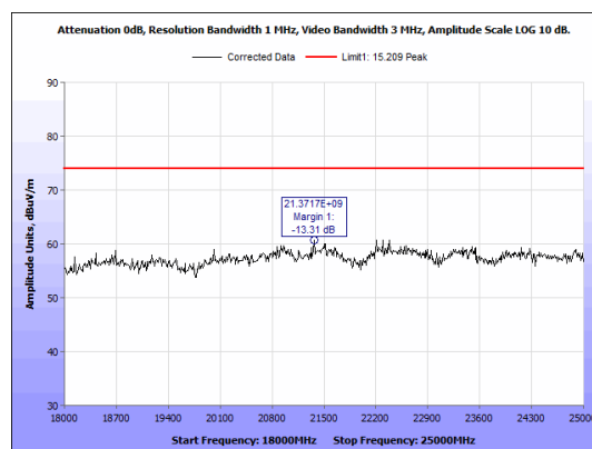
Figure 39: Radiated Emission Peak. BLE 1 Mbps High Channel 18GHz-25GHz
