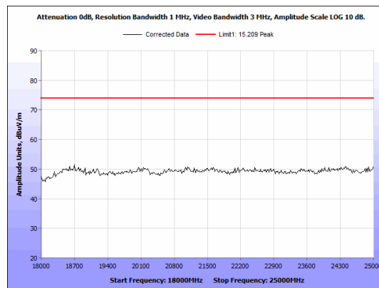
Figure 44: Radiated Emission Peak. BLE 2 Mbps Low Channel 18GHz-25GHz
