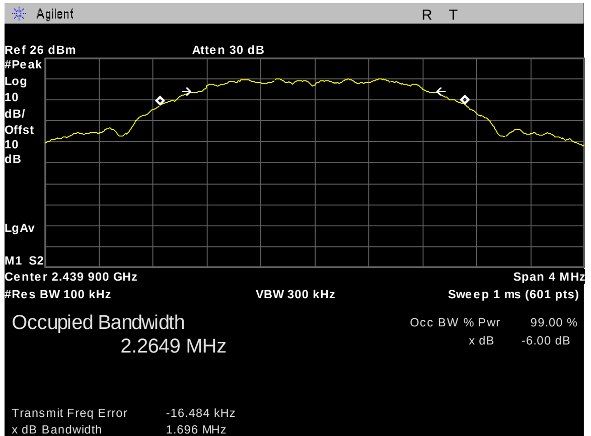
Figure 16: 6 dB Bandwidth, Mid Channel, 2440 MHz
