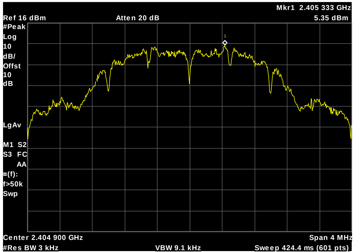
Figure 53: Peak Power Spectral Density, Low Channel, 2405 MHz
