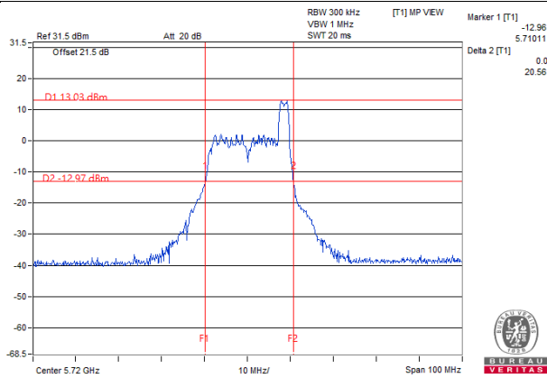
20MHz Preamble_RU106_Chain 1 / CH144 (U-NII-2C)
