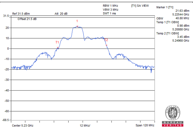
40MHz Preamble_RU106_Chain 1 / CH46
