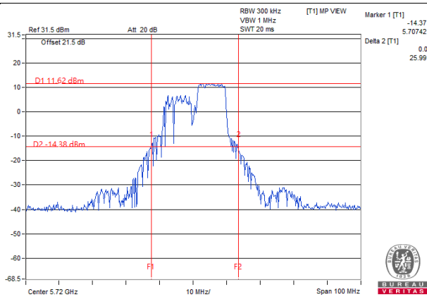
40MHz Preamble_RU26_Chain 1 / CH142 (U-NII-2C)
