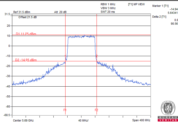
802.11ax (HE80) / Chain0 : CH138 (U-NII-2C Band)
