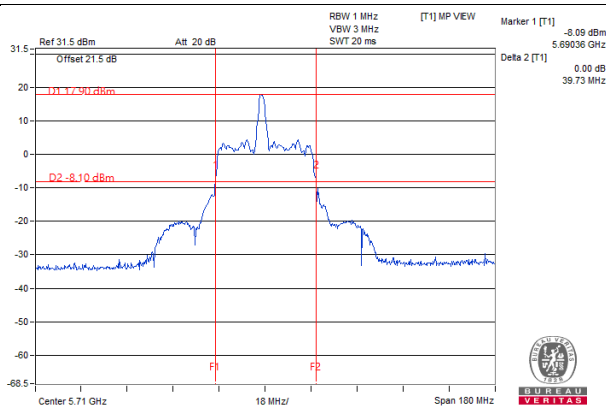
40MHz Preamble_RU106_Chain 1 / CH142 (U-NII-2C)
