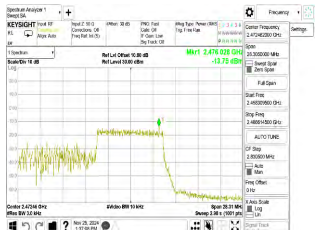
802.11ax_20MHz_Chain0_2467MHz_RU106_54
