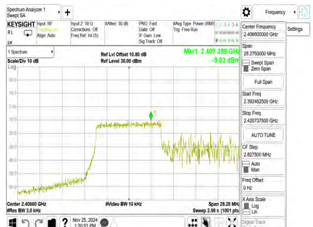
802.11ax_20MHz_Chain0_2412MHz_RU106_53
