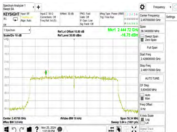
802.11ax_40MHz_Chain0_2457MHz_RU242_62
