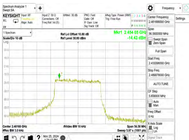
802.11ax_40MHz_Chain0_2452MHz_RU242_62
