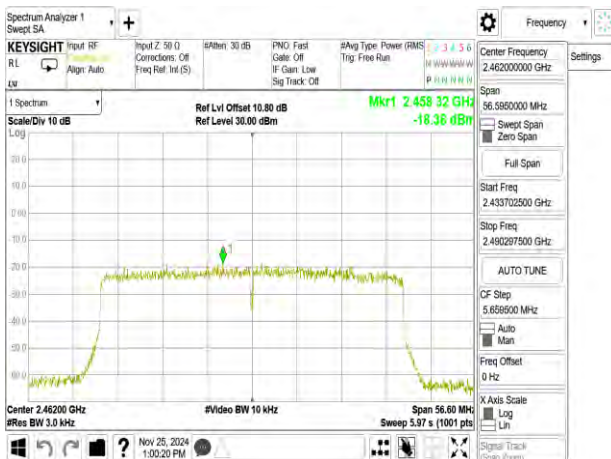
802.11ax_40MHz_Chain0_2462MHz_RU242_62
