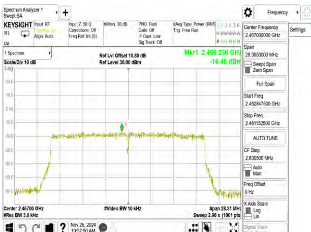
802.11ax_20MHz_Chain0_2467MHz
