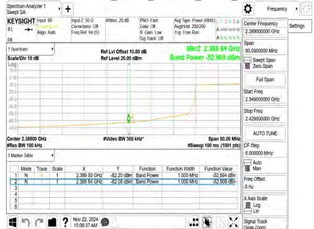
802.11ax_40MHz_2432MHz_RU484
