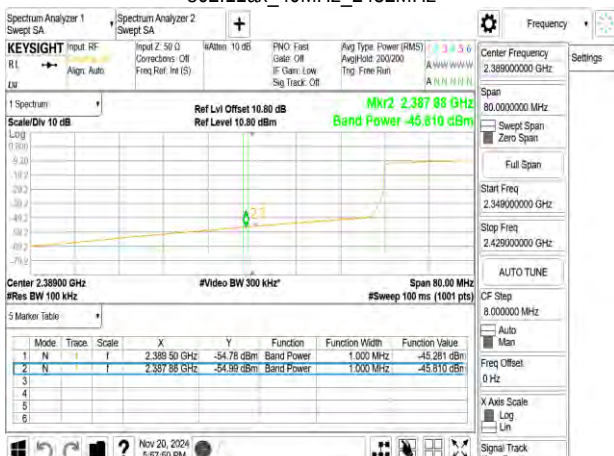
802.11ax_40MHz_2432MHz
