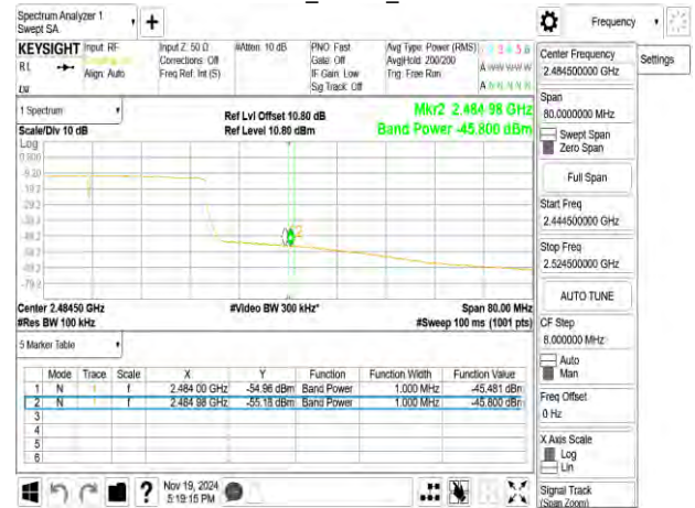
802.11ax_40MHz_2452MHz_RU242_62
