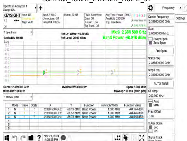
802.11ax_40MHz_2422MHz_RU242_61
