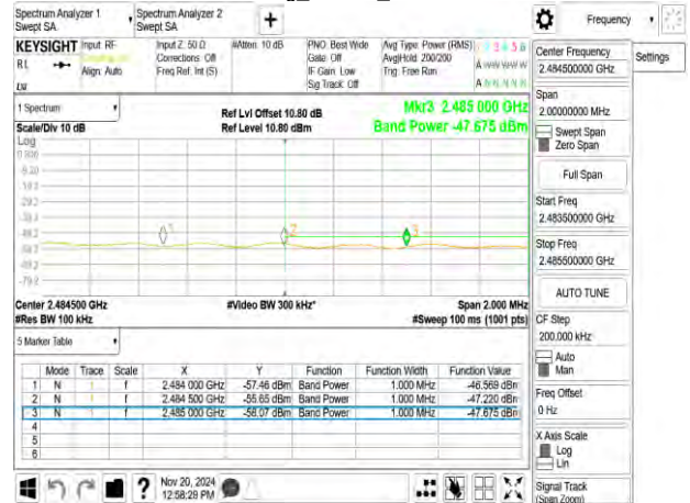
802.11g_20MHz_2467MHz
