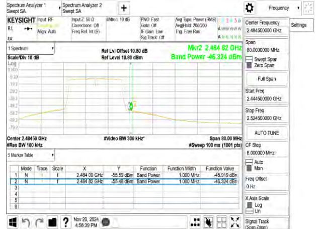
802.11ax_20MHz_2472MHz_RU106_54
