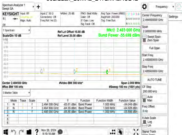
802.11ax_20MHz_2472MHz_RU106_54
