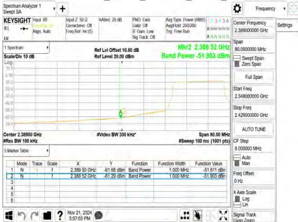
802.11ax_40MHz_2427MHz_RU484
