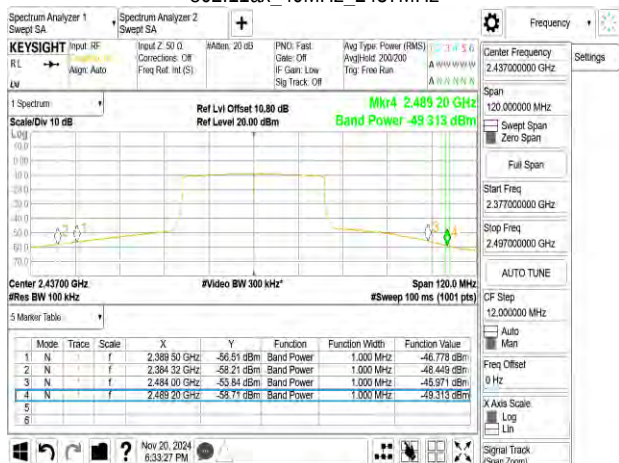
802.11ax_40MHz_2437MHz_RU242_61
