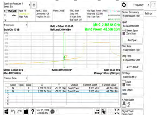
802.11ax_40MHz_2422MHz_RU484
