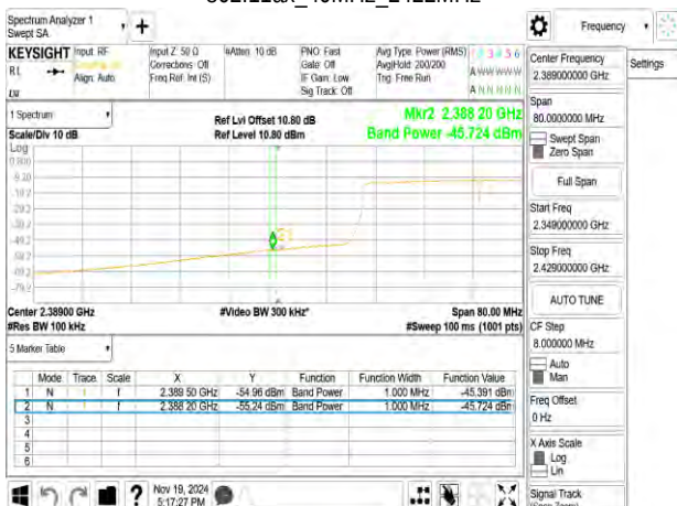
802.11ax_40MHz_2422MHz
