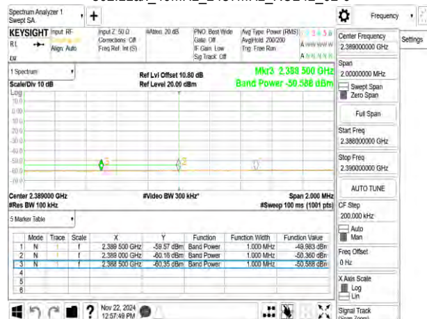
802.11ax_40MHz_2437MHz_RU242_62-0
