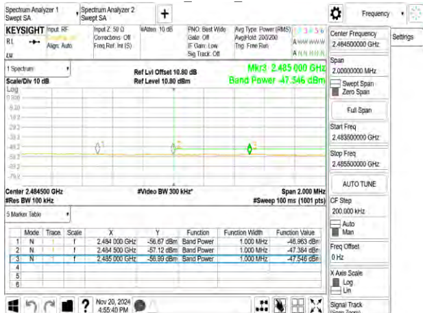
802.11ax_20MHz_2467MHzRU242
