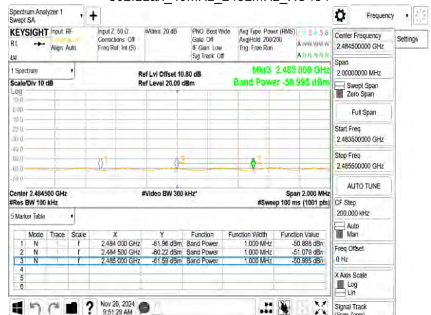
802.11ax_40MHz_2452MHz_RU484
