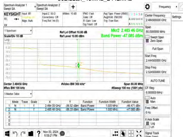
802.11ax_40MHz_2442MHz_RU242_62
