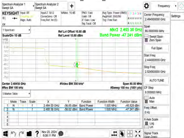
802.11ax_40MHz_2447MHz_RU242_62
