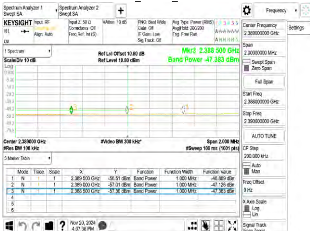
802.11ax_20MHz_2432MHz
