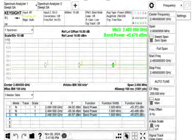
802.11ax_40MHz_2452MHz_RU242_62
