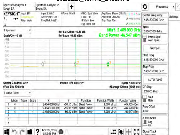
802.11ax_40MHz_2462MHz_RU242_62
