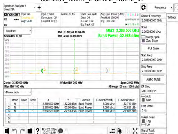
802.11ax_40MHz_2432MHz_RU242_61
