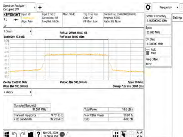
802.11ax_40MHz_Chain0_2462MHz
