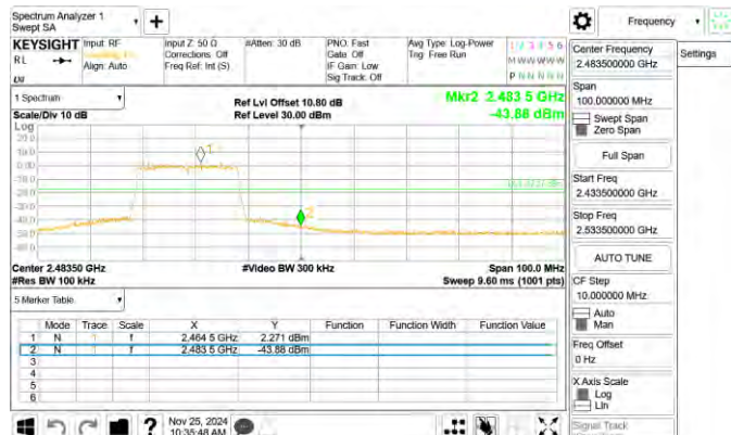
802.11ax_20MHz_Chain0_2462MHz_RU106_54
