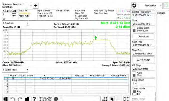
802.11ax_20MHz_Chain0_2472MHz_RU106_54
