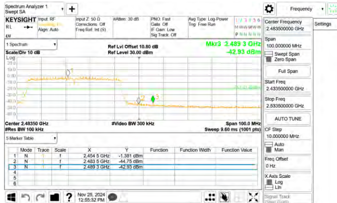
802.11ax_40MHz_Chain0_2457MHz_RU242_62
