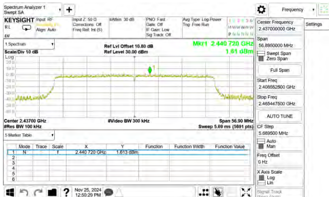
802.11ax_40MHz_Chain0_2437MHz_RU242_61
