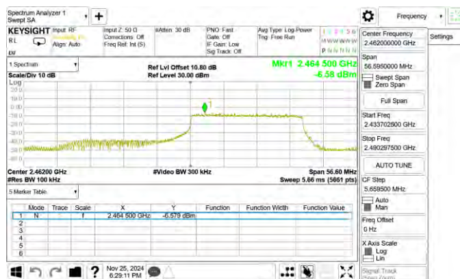
802.11ax_40MHz_Chain0_2462MHz_RU242_62
