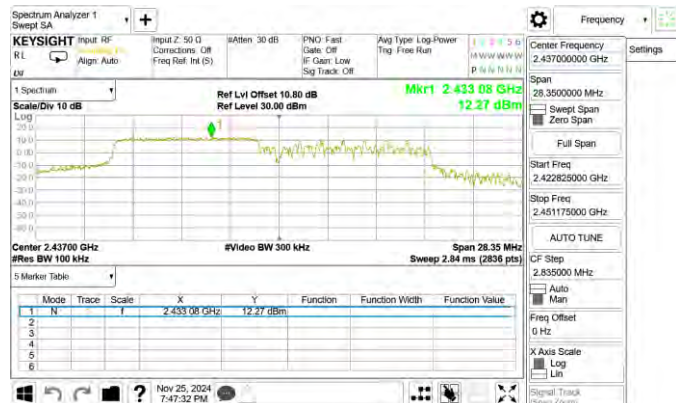
802.11ax_20MHz_Chain0_2437MHz_RU106_54
