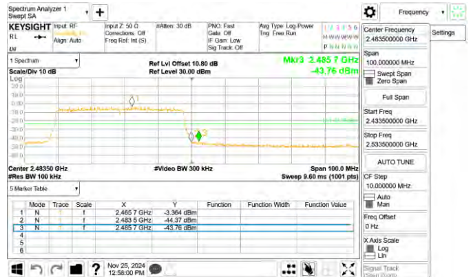
802.11ax_40MHz_Chain0_2462MHz_RU242_62
