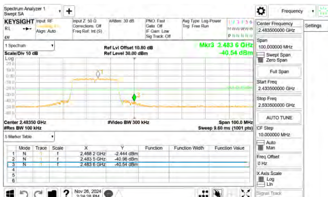
802.11ax_20MHz_Chain0_2467MHz_RU26_8
