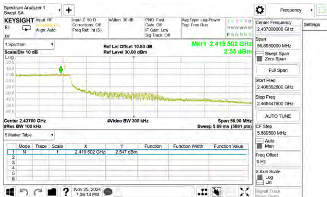
802.11ax_40MHz_Chain0_2437MHz_RU242_62
