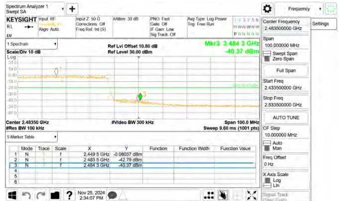
802.11ax_40MHz_Chain0_2452MHz_RU242_62
