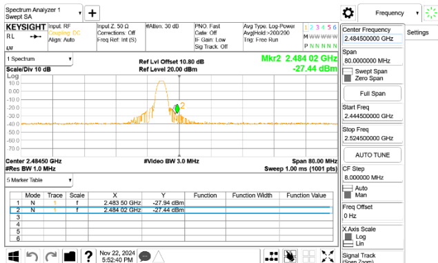
CBE_BLE_125k_2480MHz
