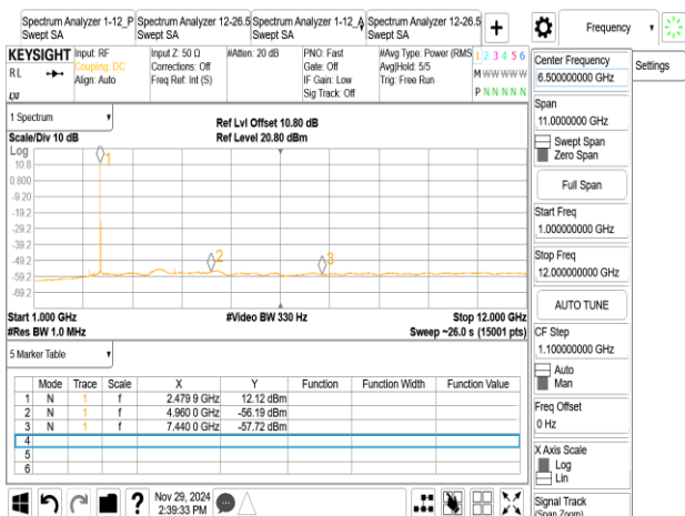
BLE_125k_2480MHz
