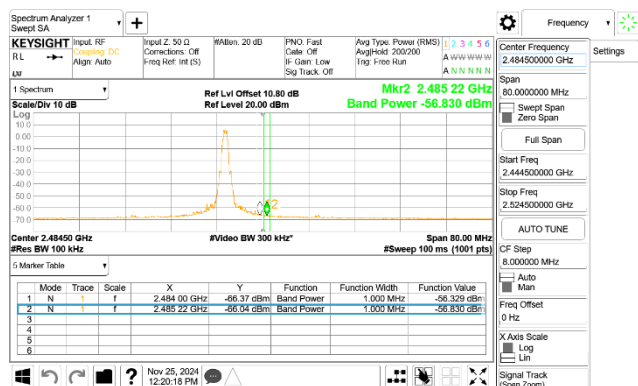
CBE_BLE_125k_2480MHz
