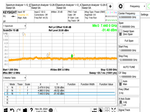
BLE_500k_2480MHz
