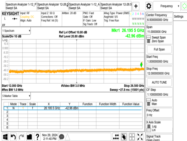
BLE_125k_2442MHz
