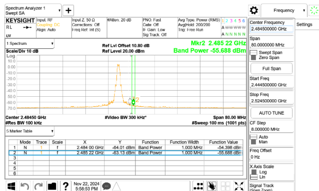
CBE_BLE_125k_2480MHz
