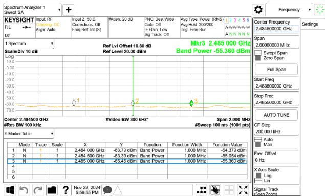
CBE_BLE_125k_2480MHz
