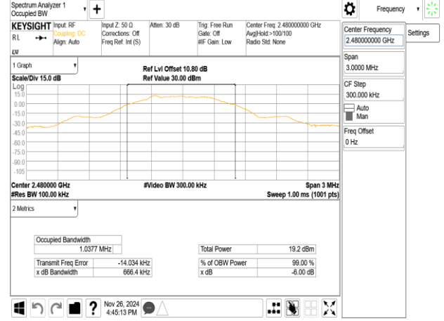
OBW_BLE 500k_HighCH39-2480MHz
