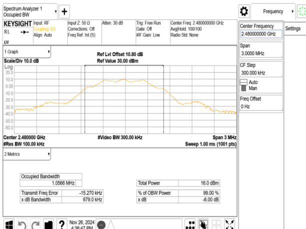
OBW_BLE 125k_HighCH39-2480MHz
