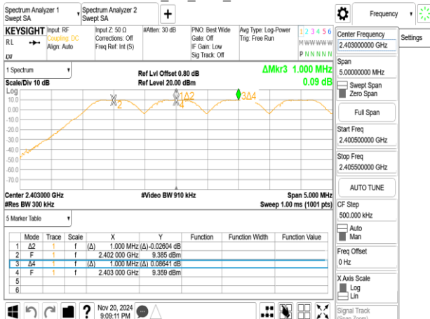
GFSK_1M_DH5_CH38CH39CH40
