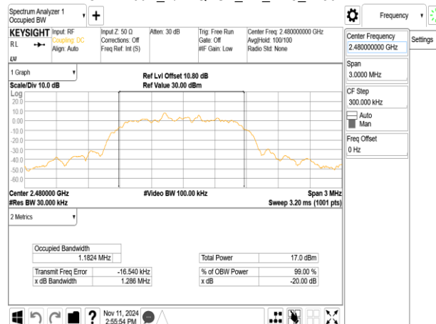
OBW 20dB_π/4DQPSK_2M_DH5_2480MHz
