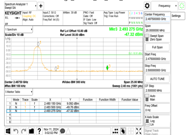
Band Edge_8DPSK_3M_DH5_2480MHz
