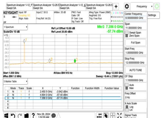
802.11ax_40MHz_2452MHz_RU484
