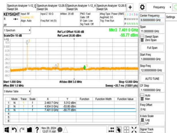
802.11ax_20MHz_2467MHz_RU26_8
