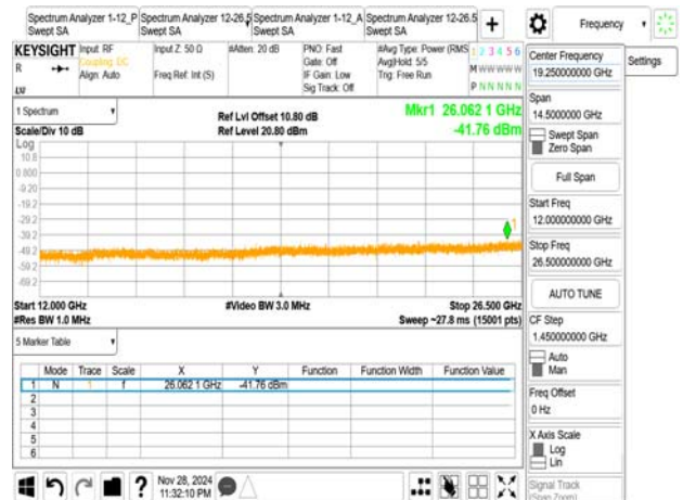
802.11ax_20MHz_2467MHz_RU52_40
