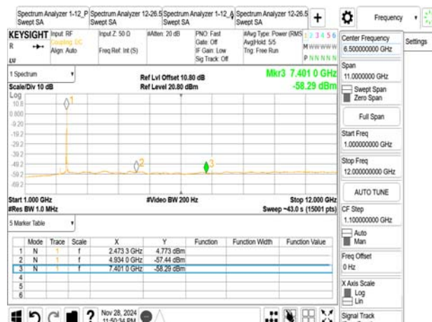
802.11ax_20MHz_2467MHz_RU52_40
