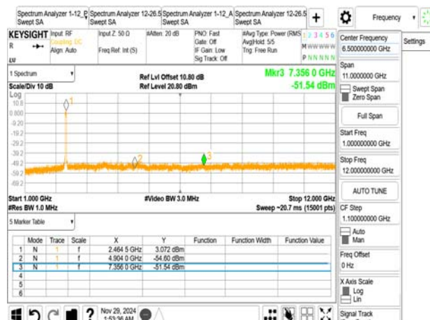
802.11ax_40MHz_2452MHz_RU484
