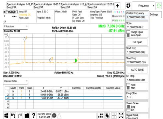
802.11ax_40MHz_2452MHz_RU242_62
