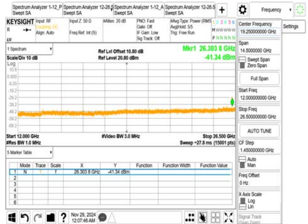
802.11ax_20MHz_2467MHz_RU26_8
