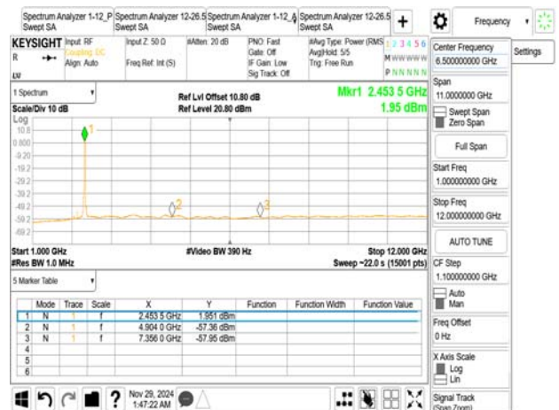
802.11ax_40MHz_2452MHz_RU484
