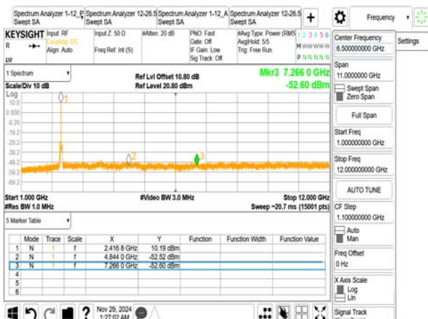
802.11ax_40MHz_2422MHz_RU484
