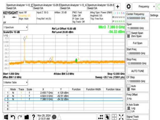
802.11ax_40MHz_2462MHz_RU242_62
