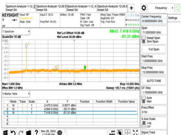
802.11ax_20MHz_2472MHz_RU242
