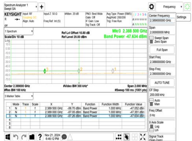
802.11ax_20MHz_2422MHz_RU242
