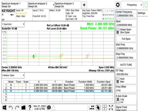
802.11ax_40MHz_2437MHz_RU242_62_R
