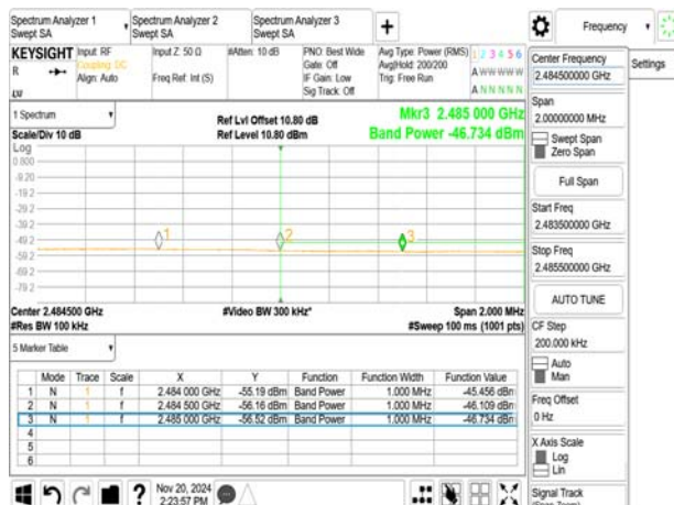
802.11ax_20MHz_2472MHz_RU106_54
