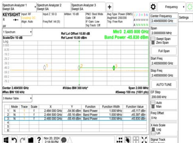
802.11ax_20MHz_2462MHz_RU106_54
