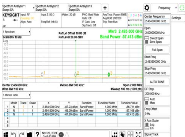
802.11ax_20MHz_2467MHz_RU26_8
