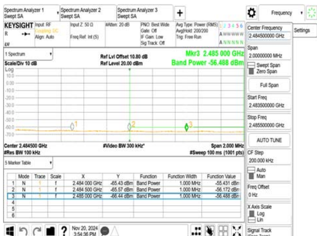
802.11ax_20MHz_2467MHz_RU242
