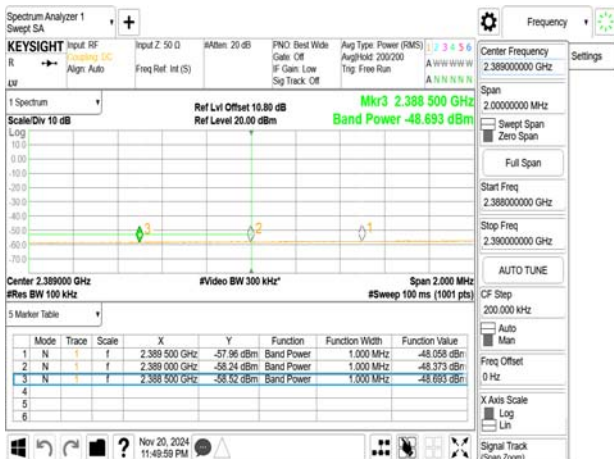
802.11ax_20MHz_2432MHz_RU106_53
