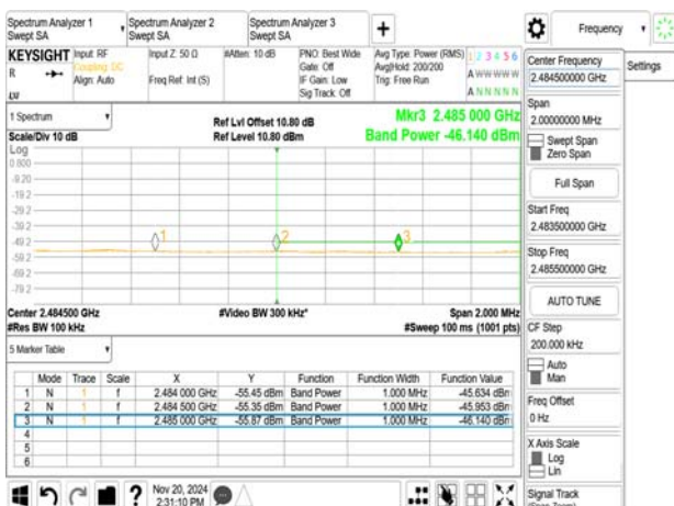
802.11ax_40MHz_2442MHz
