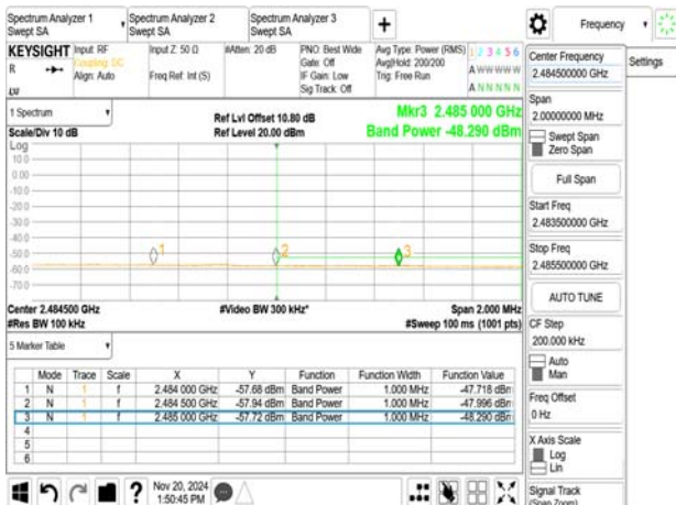
802.11ax_40MHz_2437MHz_RU484_L
