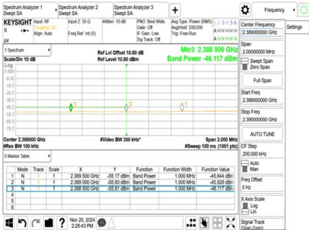
802.11ax_40MHz_2427MHz_RU242_61
