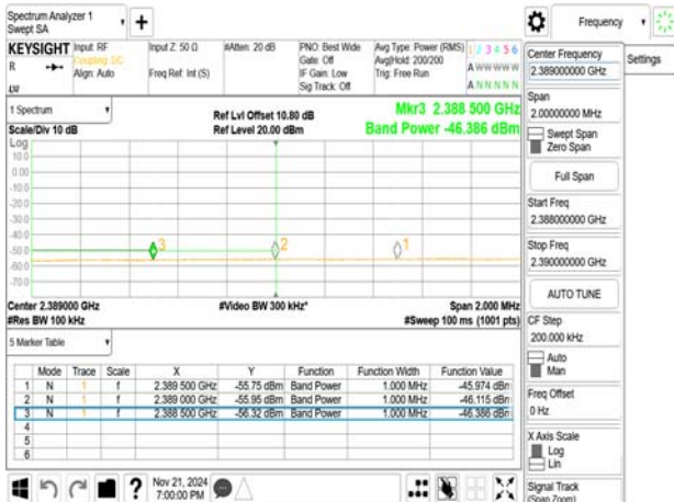
802.11ax_20MHz_2432MHz
