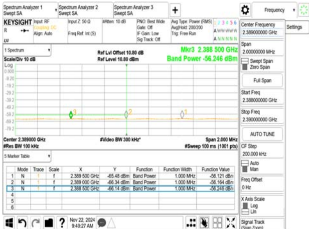
802.11ax_20MHz_2437MHz_RU106_54_R
