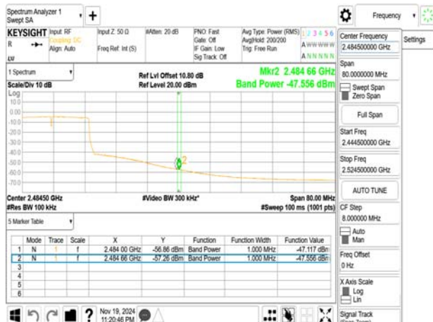
802.11ax_20MHz_2452MHz_RU106_54
