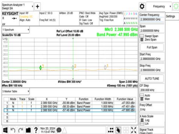
802.11g_20MHz_2432MHz
