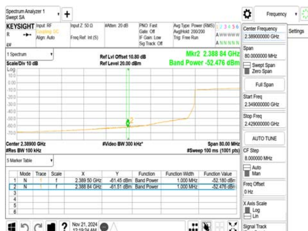
802.11ax_40MHz_2432MHz_RU242_61
