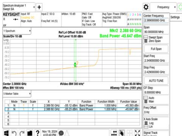
802.11ax_40MHz_2422MHz_RU242_61
