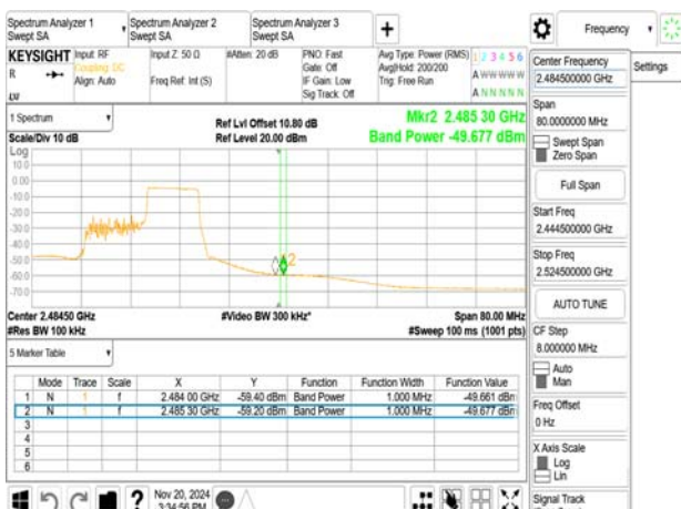
802.11ax_20MHz_2462MHz_RU106_54
