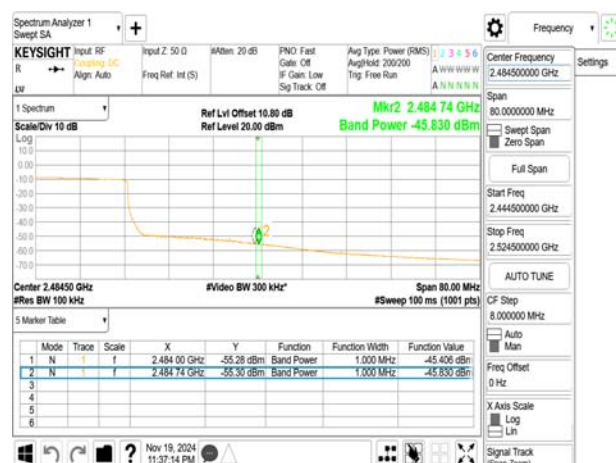
802.11ax_40MHz_2442MHz
