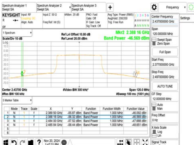
802.11ax_40MHz_2437MHz_RU242_61
