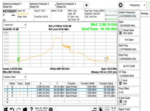
802.11ax_20MHz_2437MHz_RU106_54
