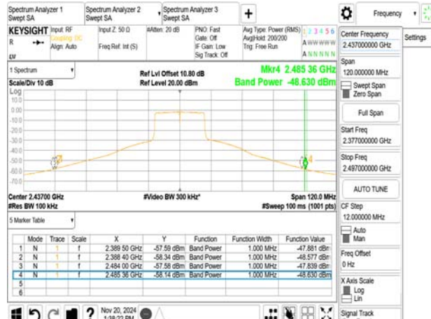
802.11ax_20MHz_2437MHz_RU106_53
