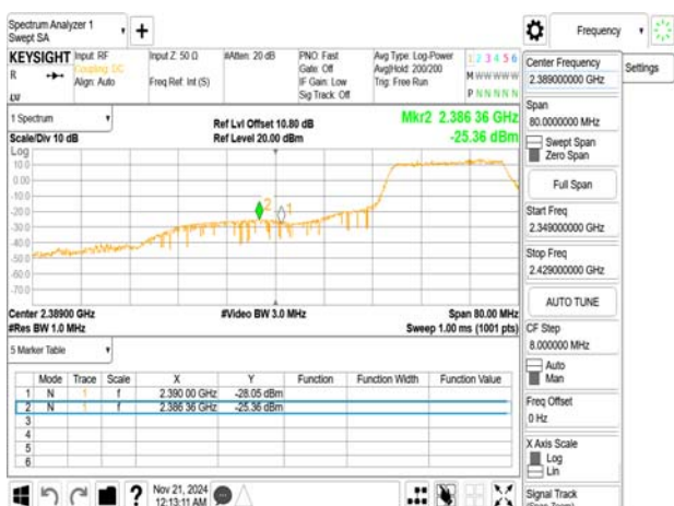
802.11ax_40MHz_2427MHz_RU242_61
