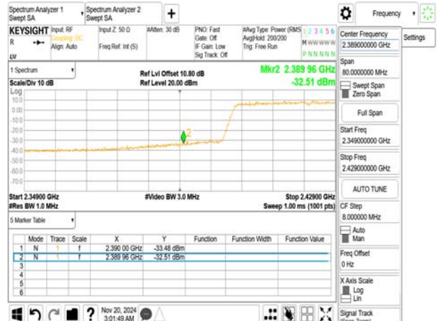
802.11ax_40MHz_2422MHz_RU242_61
