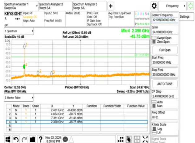
802.11ax_40MHz_Chain0_2437MHz_RU242_62
