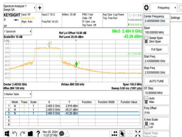
802.11ax_20MHz_Chain0_2462MHz_RU106_54
