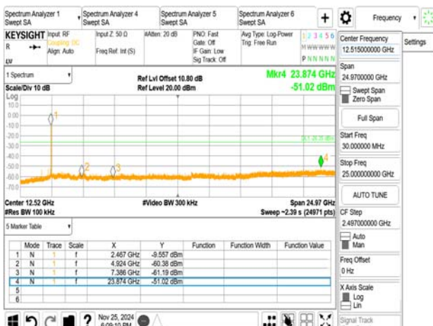
802.11ax_40MHz_Chain0_2462MHz_RU242_62
