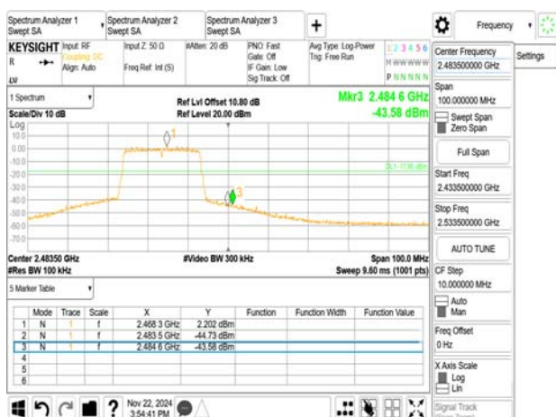
802.11ax_20MHz_Chain0_2467MHz
