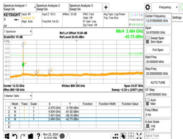
802.11ax_20MHz_Chain0_2467MHz_RU52_40
