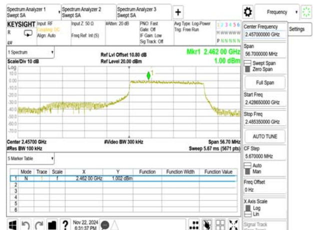
802.11ax_40MHz_Chain0_2457MHz_RU242_62
