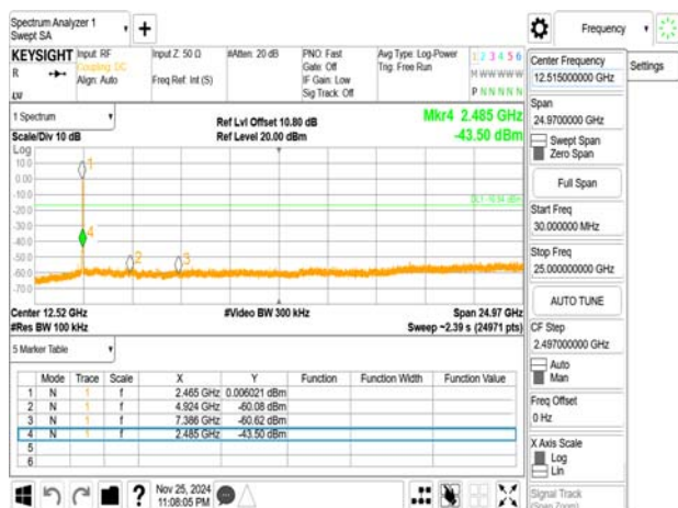
802.11ax_20MHz_Chain0_2467MHz
