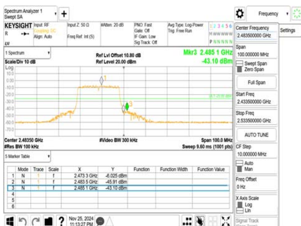
802.11ax_20MHz_Chain0_2472MHz_R242
