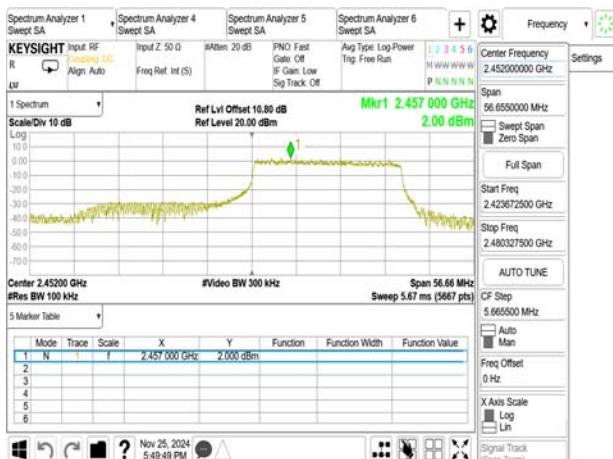
802.11ax_40MHz_Chain0_2452MHz_RU242_62
