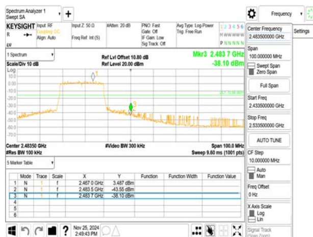
802.11ax_20MHz_Chain0_2462MHz_R242
