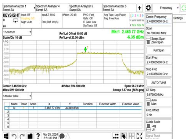
802.11ax_40MHz_Chain0_2462MHz_RU242_62
