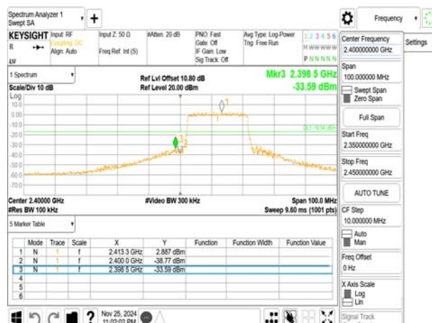
802.11ax_20MHz_Chain0_2412MHz_R242
