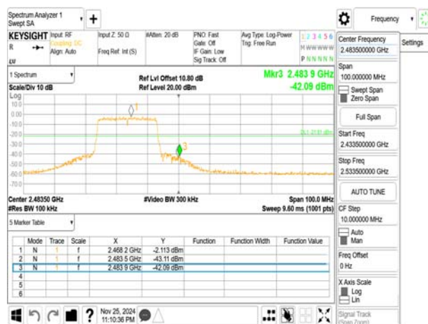
802.11ax_20MHz_Chain0_2467MHz_RU106_54
