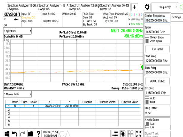
BLE_500K_2442MHz
