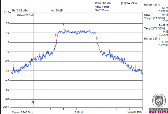
802.11ac(VHT20)_Chain2 / CH149
