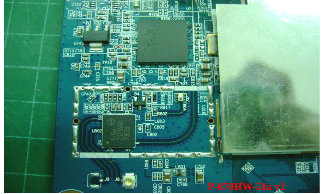
Wireless module
